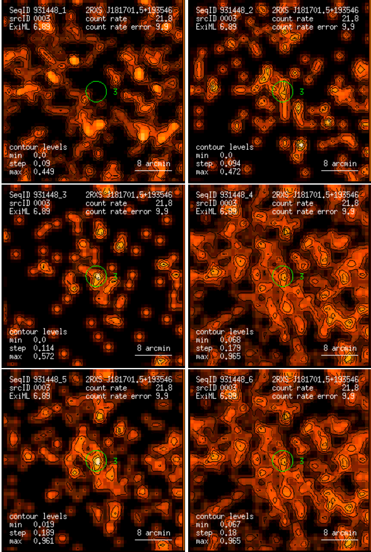
Figure 3: RASS 931448: detection 0003: band rate images, Gaussian filter: (1) PSPC channels 11 – 41, (2) 52 – 90, (3) 91 – 201, (4) 11 – 235, (5) 52 – 201, (6) 11 – 201. Broad band rates in counts/ks. Band rate contour levels in counts/ks/arcmin 2 .
