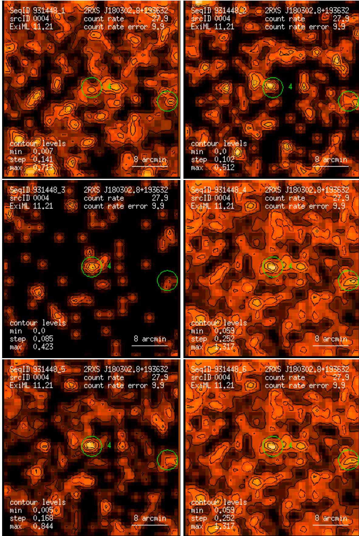
Figure 4: RASS 931448: detection 0004: band rate images, Gaussian filter: (1) PSPC channels 11 – 41, (2) 52 – 90, (3) 91 – 201, (4) 11 – 235, (5) 52 – 201, (6) 11 – 201. Broad band rates in counts/ks. Band rate contour levels in counts/ks/arcmin 2 .
