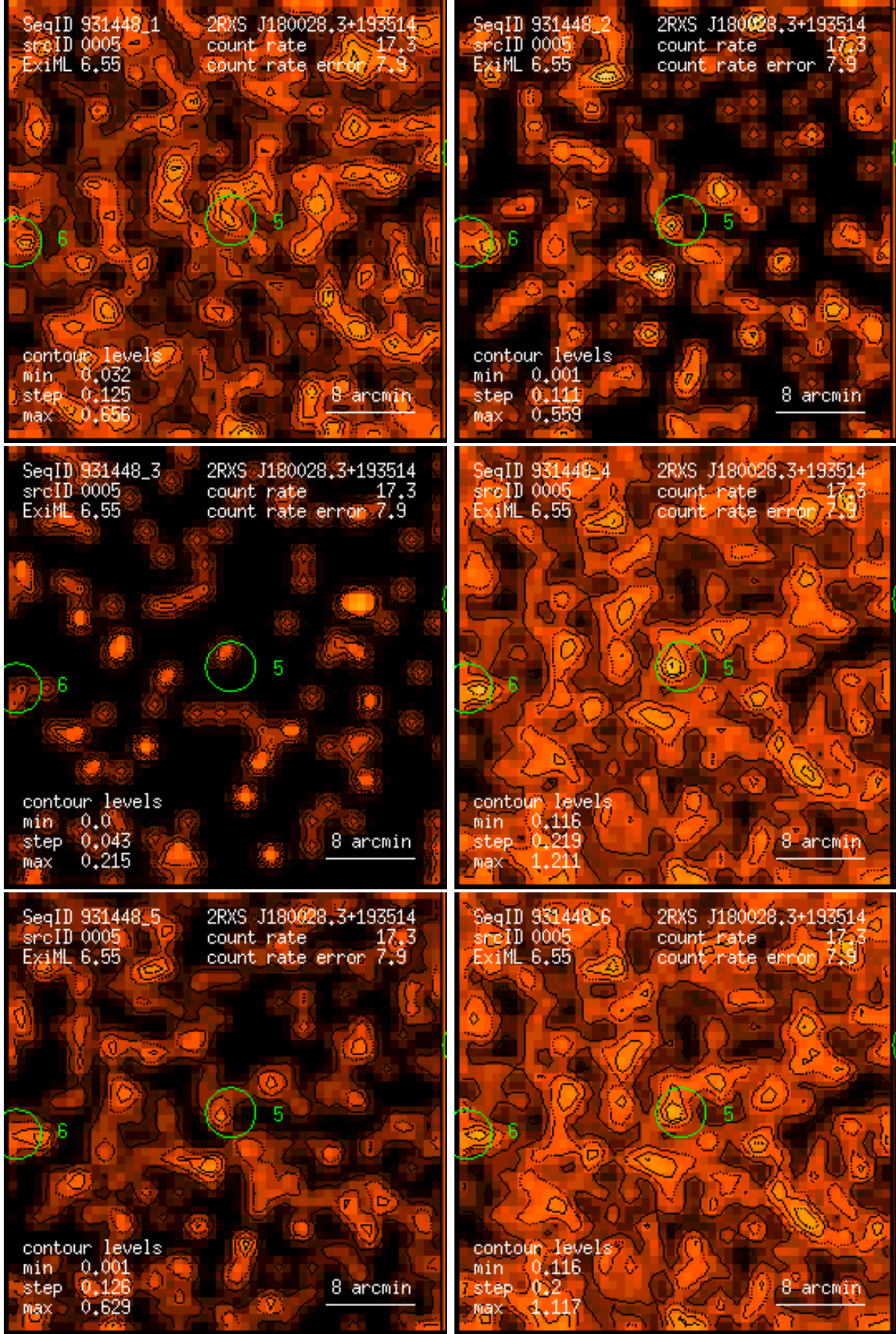
Figure 5: RASS 931448: detection 0005: band rate images, Gaussian filter: (1) PSPC channels 11 – 41, (2) 52 – 90, (3) 91 – 201, (4) 11 – 235, (5) 52 – 201, (6) 11 – 201. Broad band rates in counts/ks. Band rate contour levels in counts/ks/arcmin 2 .
