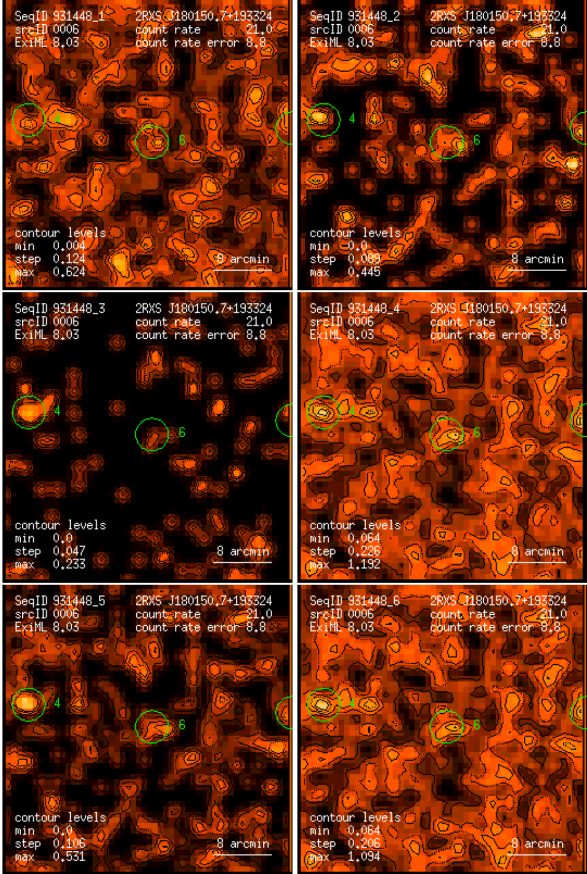
Figure 6: RASS 931448: detection 0006: band rate images, Gaussian filter: (1) PSPC channels 11 – 41, (2) 52 – 90, (3) 91 – 201, (4) 11 – 235, (5) 52 – 201, (6) 11 – 201. Broad band rates in counts/ks. Band rate contour levels in counts/ks/arcmin 2 .
