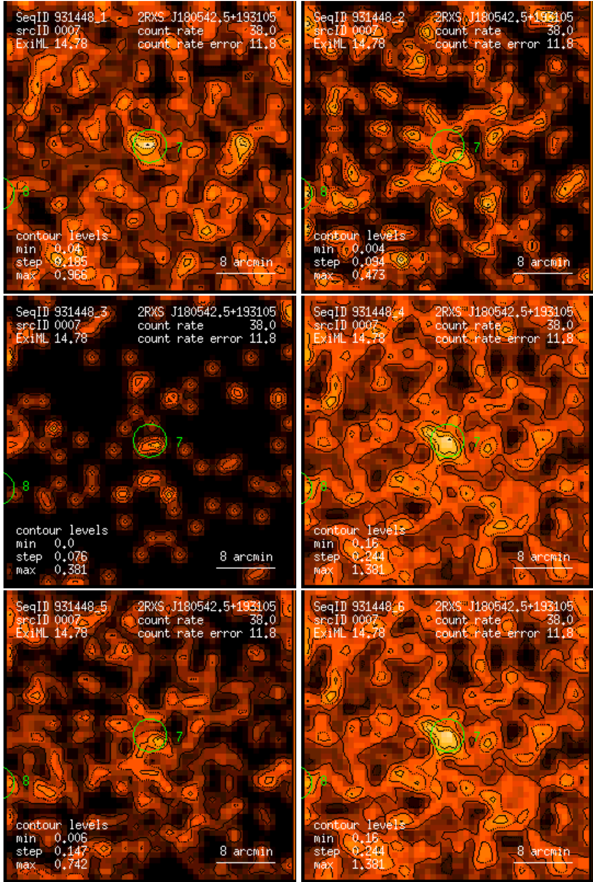
Figure 7: RASS 931448: detection 0007: band rate images, Gaussian filter: (1) PSPC channels 11 – 41, (2) 52 – 90, (3) 91 – 201, (4) 11 – 235, (5) 52 – 201, (6) 11 – 201. Broad band rates in counts/ks. Band rate contour levels in counts/ks/arcmin 2 .
