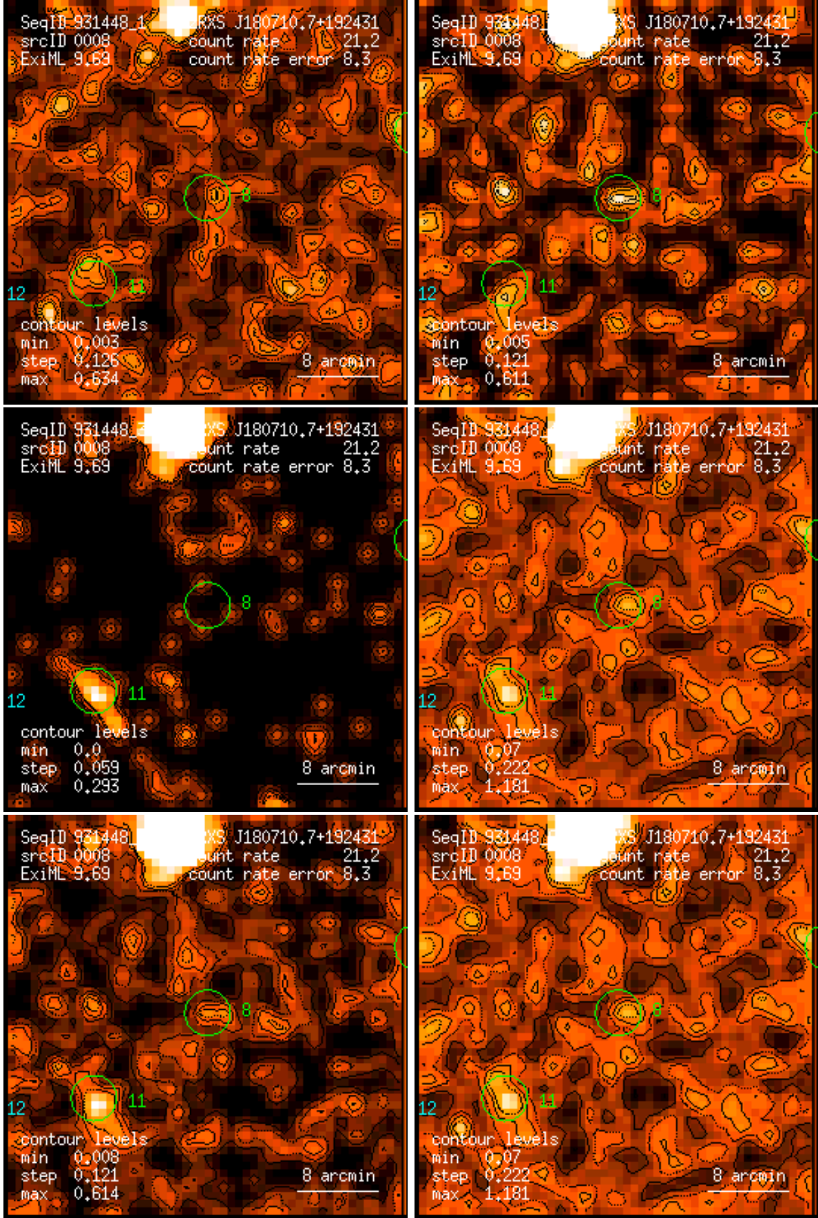
Figure 8: RASS 931448: detection 0008: band rate images, Gaussian filter: (1) PSPC channels 11 – 41, (2) 52 – 90, (3) 91 – 201, (4) 11 – 235, (5) 52 – 201, (6) 11 – 201. Broad band rates in counts/ks. Band rate contour levels in counts/ks/arcmin 2 .
