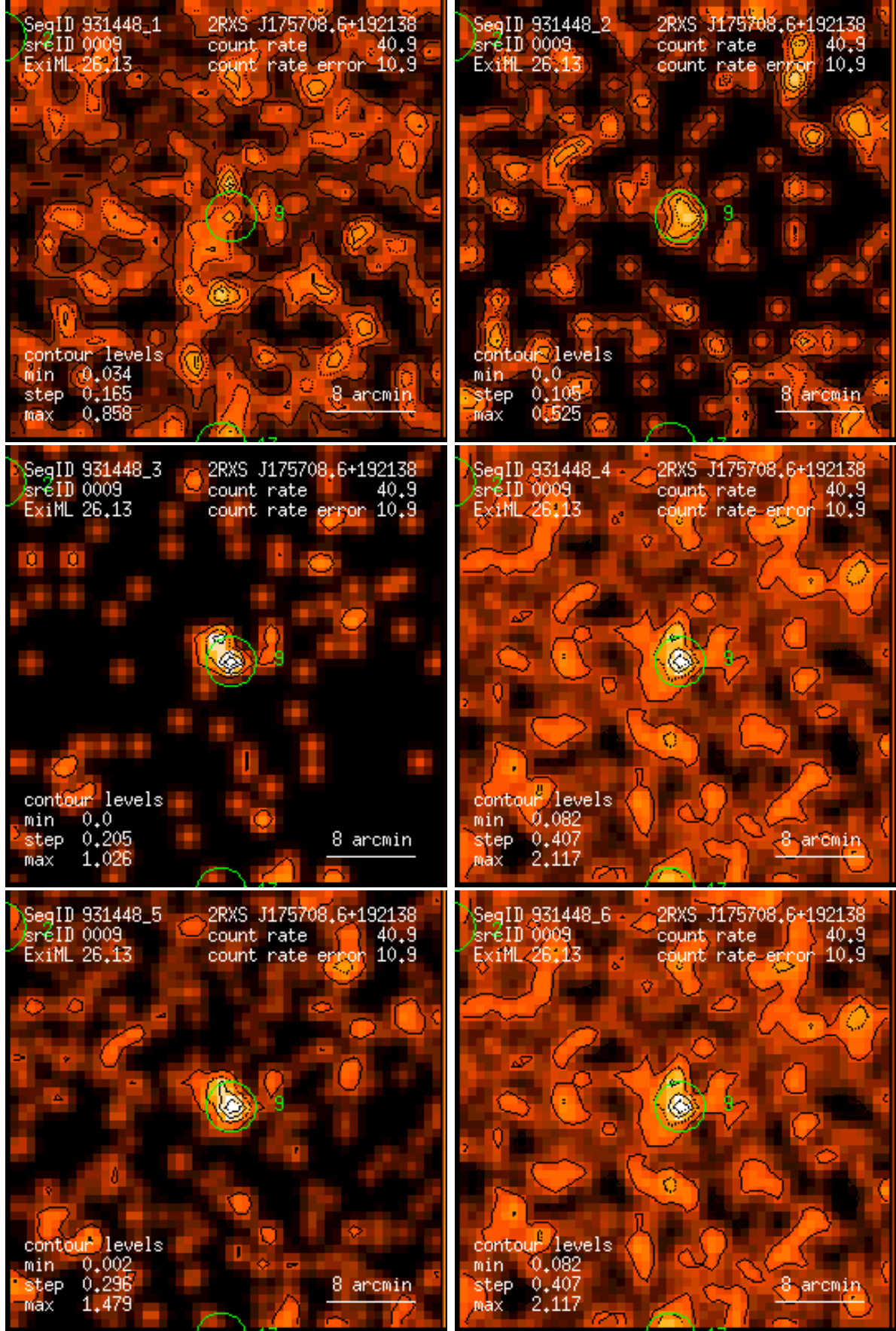
Figure 9: RASS 931448: detection 0009: band rate images, Gaussian filter: (1) PSPC channels 11 – 41, (2) 52 – 90, (3) 91 – 201, (4) 11 – 235, (5) 52 – 201, (6) 11 – 201. Broad band rates in counts/ks. Band rate contour levels in counts/ks/arcmin 2 .
