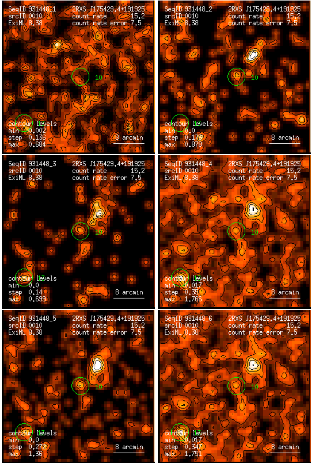
Figure 10: RASS 931448: detection 0010: band rate images, Gaussian filter: (1) PSPC channels 11 – 41, (2) 52 – 90, (3) 91 – 201, (4) 11 – 235, (5) 52 – 201, (6) 11 – 201. Broad band rates in counts/ks. Band rate contour levels in counts/ks/arcmin 2 .
