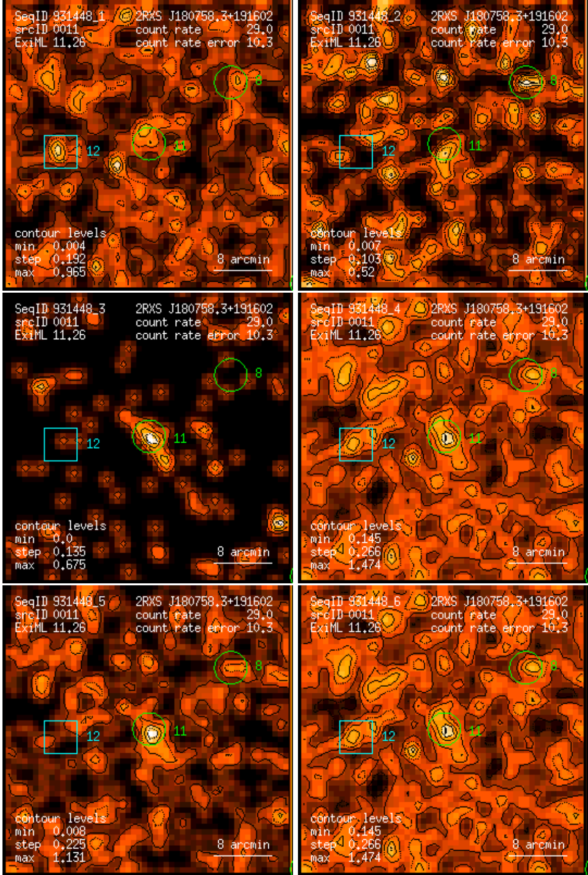
Figure 11: RASS 931448: detection 0011: band rate images, Gaussian filter: (1) PSPC channels 11 – 41, (2) 52 – 90, (3) 91 – 201, (4) 11 – 235, (5) 52 – 201, (6) 11 – 201. Broad band rates in counts/ks. Band rate contour levels in counts/ks/arcmin 2 .
