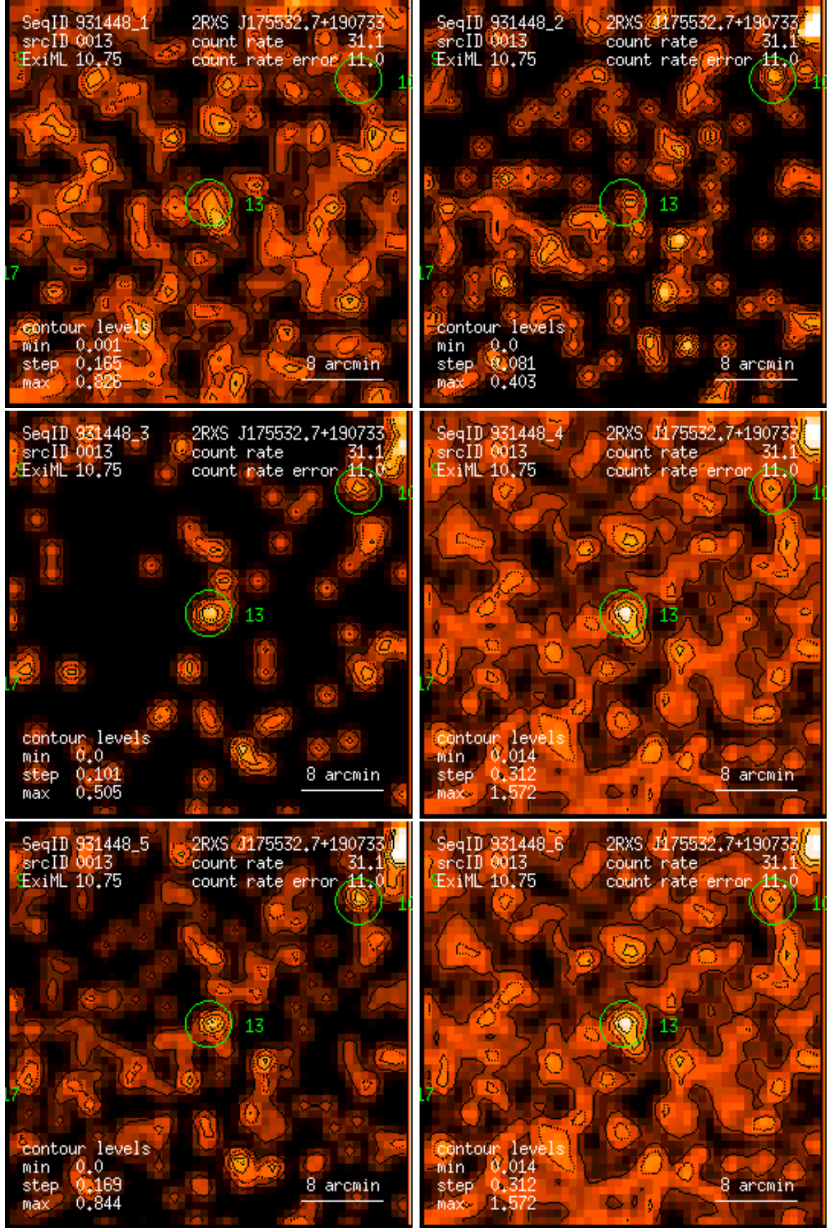
Figure 13: RASS 931448: detection 0013: band rate images, Gaussian filter: (1) PSPC channels 11 – 41, (2) 52 – 90, (3) 91 – 201, (4) 11 – 235, (5) 52 – 201, (6) 11 – 201. Broad band rates in counts/ks. Band rate contour levels in counts/ks/arcmin 2 .
