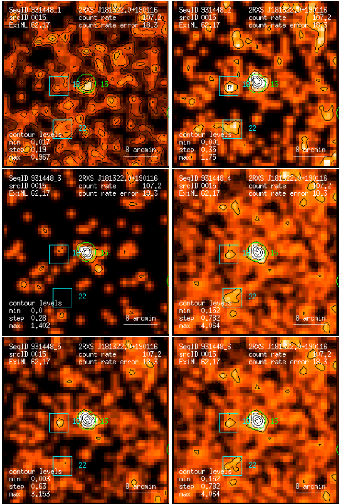
Figure 15: RASS 931448: detection 0015: band rate images, Gaussian filter: (1) PSPC channels 11 – 41, (2) 52 – 90, (3) 91 – 201, (4) 11 – 235, (5) 52 – 201, (6) 11 – 201. Broad band rates in counts/ks. Band rate contour levels in counts/ks/arcmin 2 .
