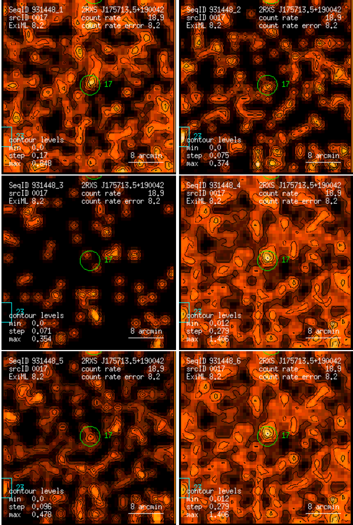
Figure 17: RASS 931448: detection 0017: band rate images, Gaussian filter: (1) PSPC channels 11 – 41, (2) 52 – 90, (3) 91 – 201, (4) 11 – 235, (5) 52 – 201, (6) 11 – 201. Broad band rates in counts/ks. Band rate contour levels in counts/ks/arcmin 2 .
