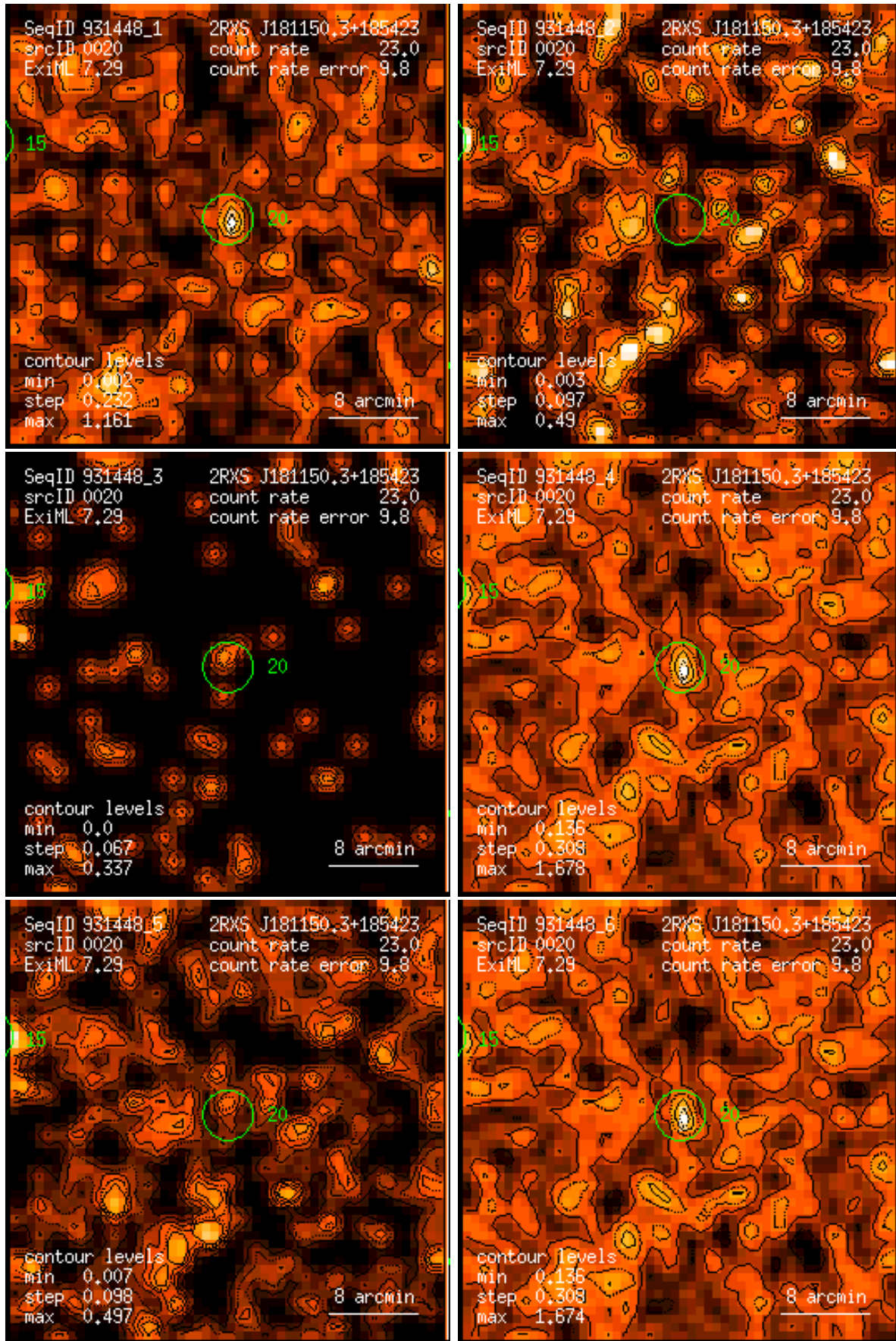
Figure 20: RASS 931448: detection 0020: band rate images, Gaussian filter: (1) PSPC channels 11 – 41, (2) 52 – 90, (3) 91 – 201, (4) 11 – 235, (5) 52 – 201, (6) 11 – 201. Broad band rates in counts/ks. Band rate contour levels in counts/ks/arcmin 2 .
