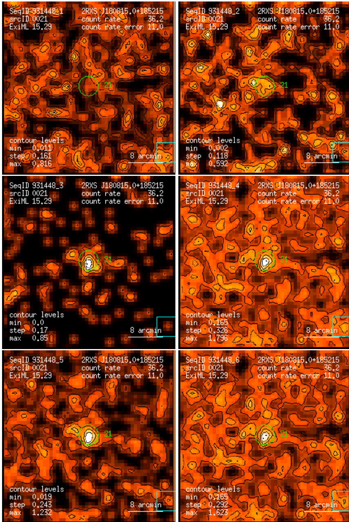
Figure 21: RASS 931448: detection 0021: band rate images, Gaussian filter: (1) PSPC channels 11 – 41, (2) 52 – 90, (3) 91 – 201, (4) 11 – 235, (5) 52 – 201, (6) 11 – 201. Broad band rates in counts/ks. Band rate contour levels in counts/ks/arcmin 2 .
