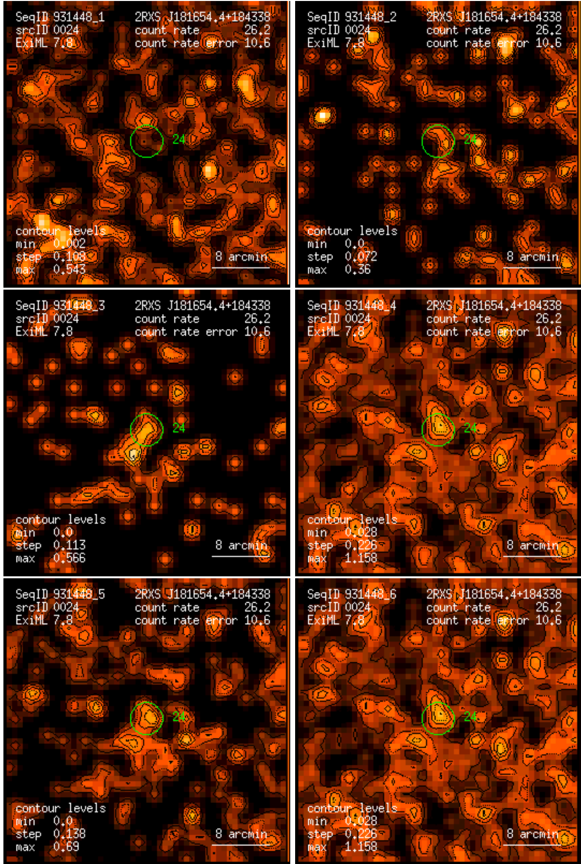
Figure 24: RASS 931448: detection 0024: band rate images, Gaussian filter: (1) PSPC channels 11 – 41, (2) 52 – 90, (3) 91 – 201, (4) 11 – 235, (5) 52 – 201, (6) 11 – 201. Broad band rates in counts/ks. Band rate contour levels in counts/ks/arcmin 2 .
