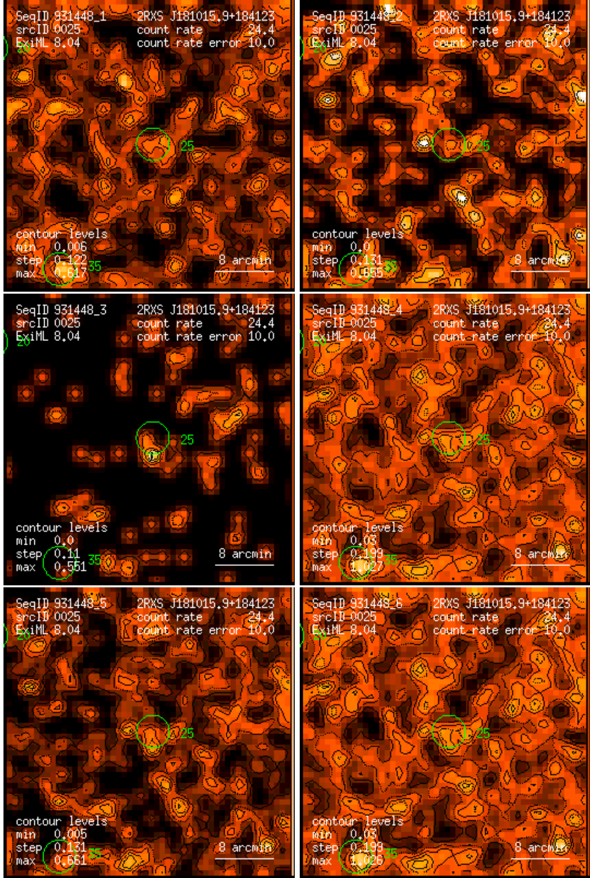
Figure 25: RASS 931448: detection 0025: band rate images, Gaussian filter: (1) PSPC channels 11 – 41, (2) 52 – 90, (3) 91 – 201, (4) 11 – 235, (5) 52 – 201, (6) 11 – 201. Broad band rates in counts/ks. Band rate contour levels in counts/ks/arcmin 2 .
