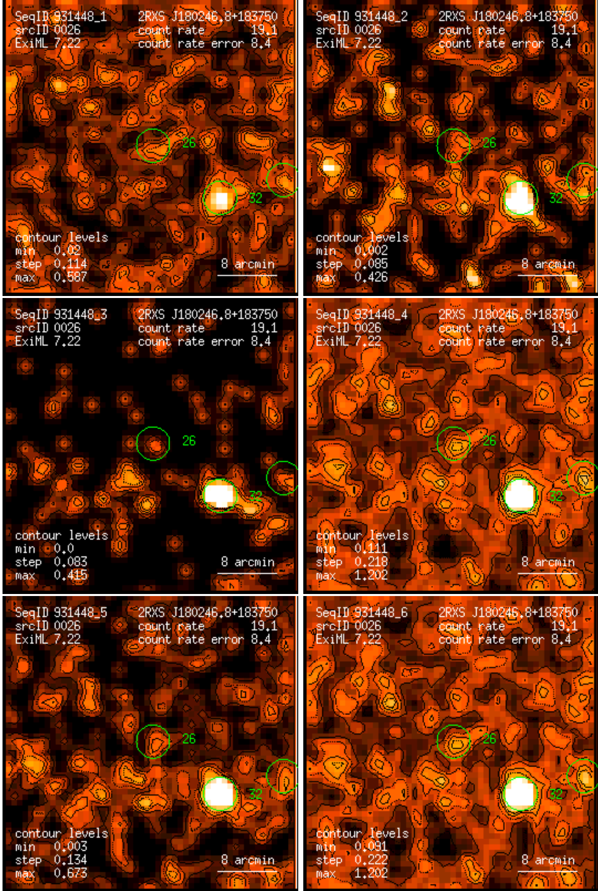
Figure 26: RASS 931448: detection 0026: band rate images, Gaussian filter: (1) PSPC channels 11 – 41, (2) 52 – 90, (3) 91 – 201, (4) 11 – 235, (5) 52 – 201, (6) 11 – 201. Broad band rates in counts/ks. Band rate contour levels in counts/ks/arcmin 2 .
