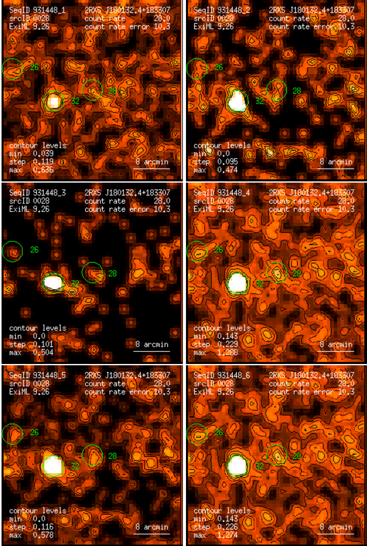
Figure 28: RASS 931448: detection 0028: band rate images, Gaussian filter: (1) PSPC channels 11 – 41, (2) 52 – 90, (3) 91 – 201, (4) 11 – 235, (5) 52 – 201, (6) 11 – 201. Broad band rates in counts/ks. Band rate contour levels in counts/ks/arcmin 2 .
