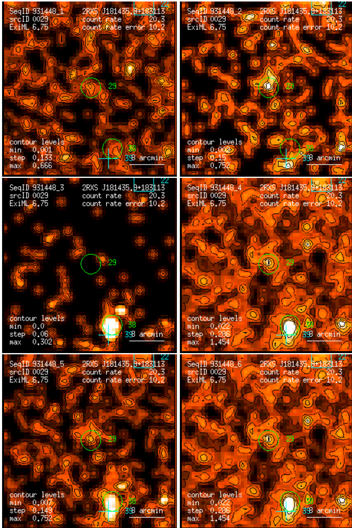
Figure 29: RASS 931448: detection 0029: band rate images, Gaussian filter: (1) PSPC channels 11 – 41, (2) 52 – 90, (3) 91 – 201, (4) 11 – 235, (5) 52 – 201, (6) 11 – 201. Broad band rates in counts/ks. Band rate contour levels in counts/ks/arcmin 2 .
