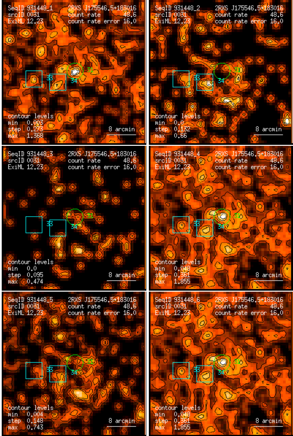
Figure 31: RASS 931448: detection 0031: band rate images, Gaussian filter: (1) PSPC channels 11 – 41, (2) 52 – 90, (3) 91 – 201, (4) 11 – 235, (5) 52 – 201, (6) 11 – 201. Broad band rates in counts/ks. Band rate contour levels in counts/ks/arcmin 2 .
