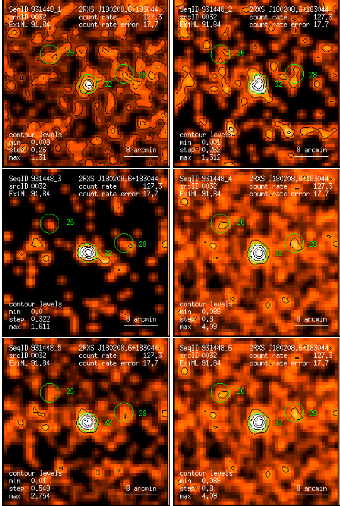
Figure 32: RASS 931448: detection 0032: band rate images, Gaussian filter: (1) PSPC channels 11 – 41, (2) 52 – 90, (3) 91 – 201, (4) 11 – 235, (5) 52 – 201, (6) 11 – 201. Broad band rates in counts/ks. Band rate contour levels in counts/ks/arcmin 2 .
