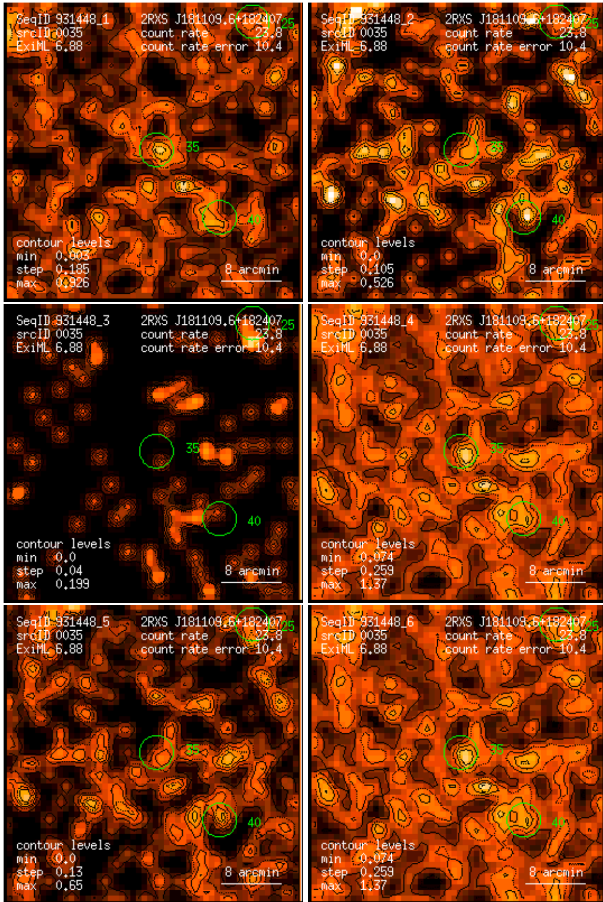
Figure 35: RASS 931448: detection 0035: band rate images, Gaussian filter: (1) PSPC channels 11 – 41, (2) 52 – 90, (3) 91 – 201, (4) 11 – 235, (5) 52 – 201, (6) 11 – 201. Broad band rates in counts/ks. Band rate contour levels in counts/ks/arcmin 2 .
