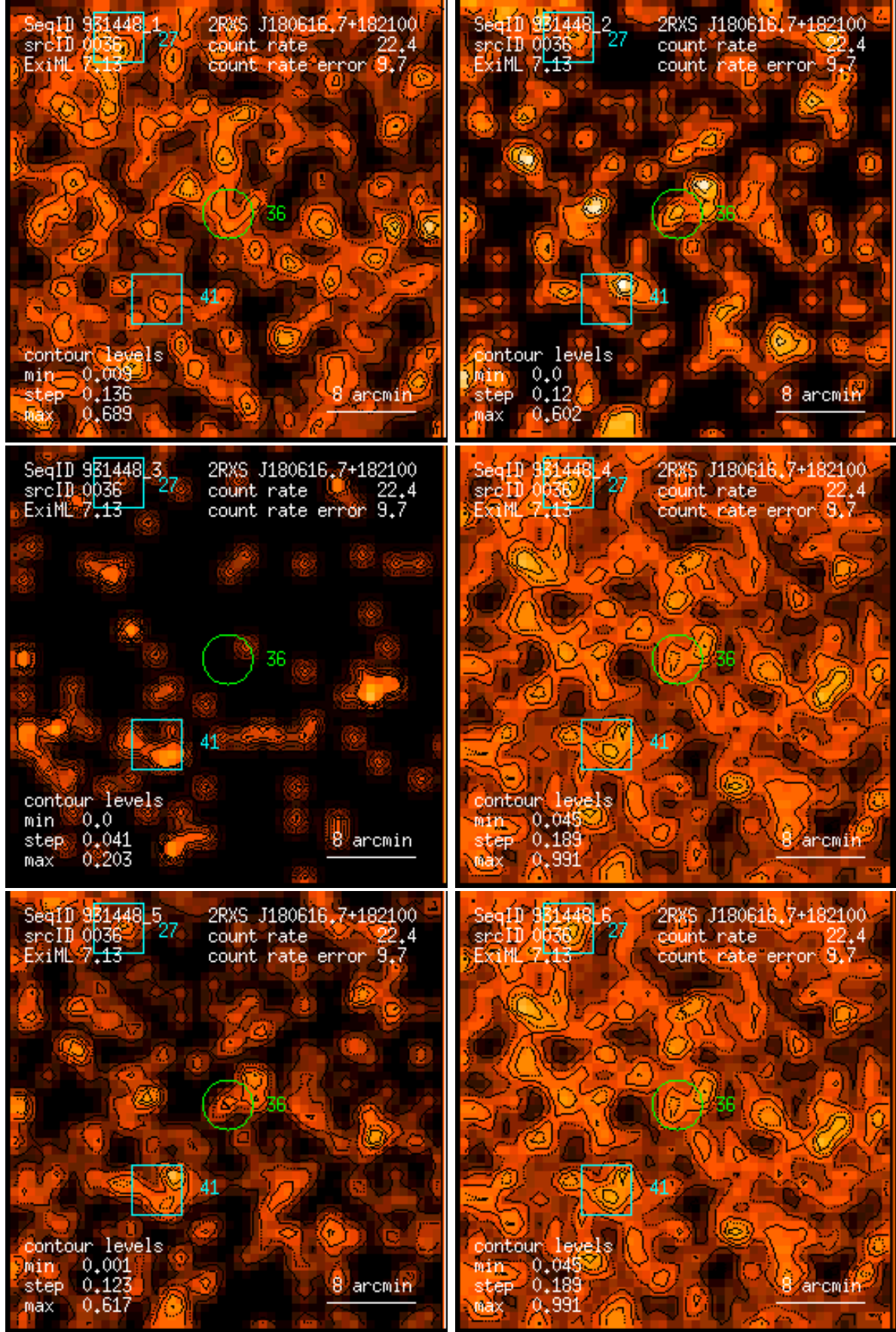
Figure 36: RASS 931448: detection 0036: band rate images, Gaussian filter: (1) PSPC channels 11 – 41, (2) 52 – 90, (3) 91 – 201, (4) 11 – 235, (5) 52 – 201, (6) 11 – 201. Broad band rates in counts/ks. Band rate contour levels in counts/ks/arcmin 2 .
