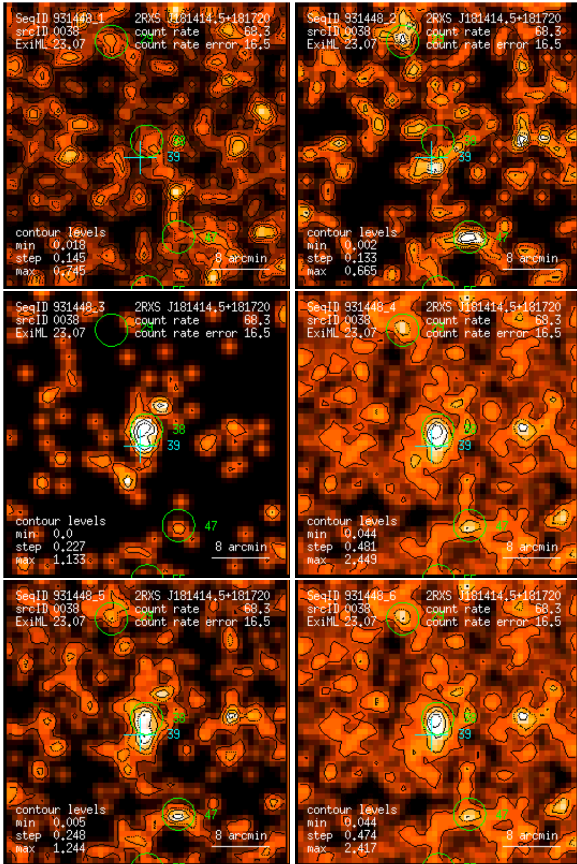
Figure 38: RASS 931448: detection 0038: band rate images, Gaussian filter: (1) PSPC channels 11 – 41, (2) 52 – 90, (3) 91 – 201, (4) 11 – 235, (5) 52 – 201, (6) 11 – 201. Broad band rates in counts/ks. Band rate contour levels in counts/ks/arcmin 2 .
