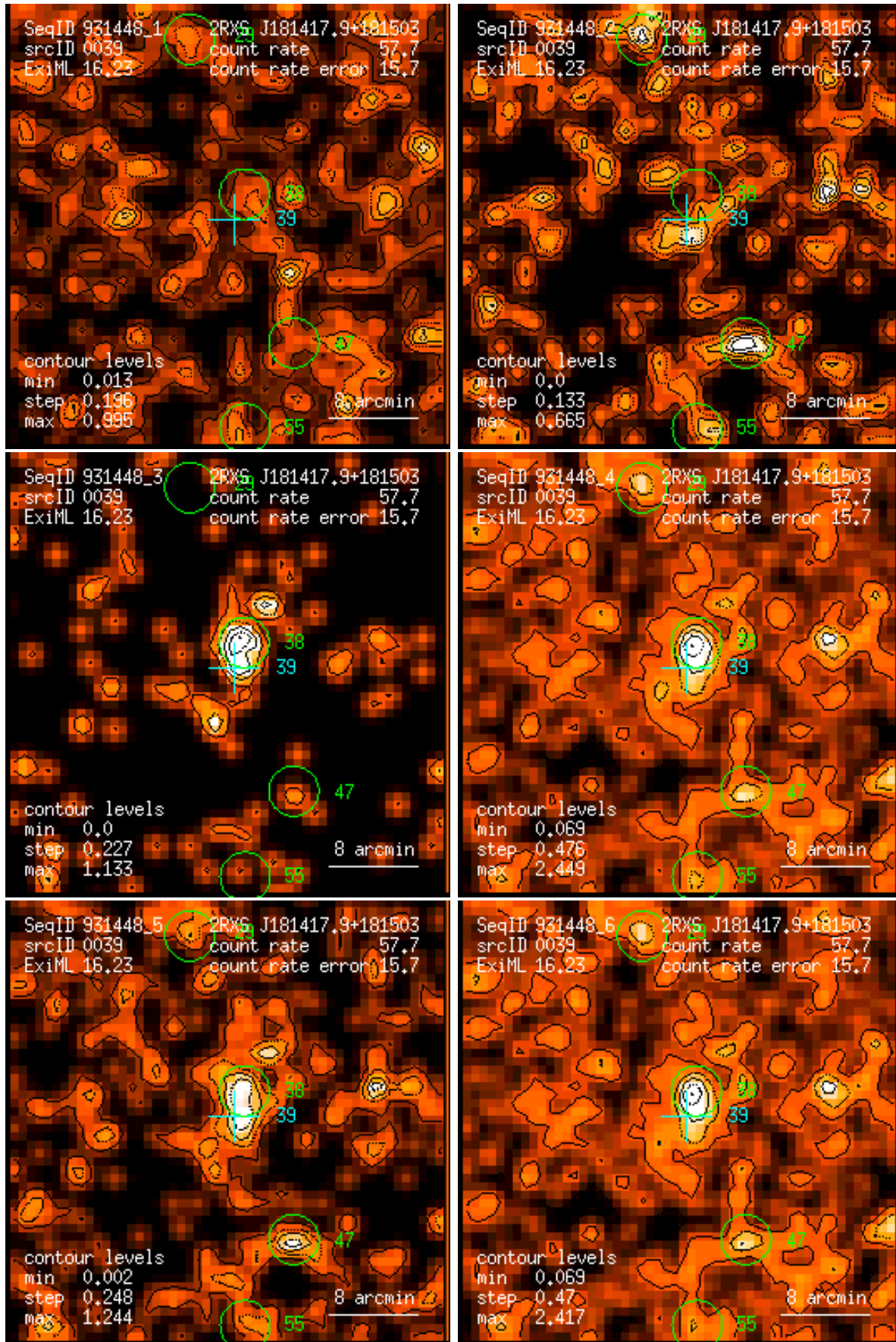
Figure 39: RASS 931448: detection 0039: band rate images, Gaussian filter: (1) PSPC channels 11 – 41, (2) 52 – 90, (3) 91 – 201, (4) 11 – 235, (5) 52 – 201, (6) 11 – 201. Broad band rates in counts/ks. Band rate contour levels in counts/ks/arcmin 2 .
