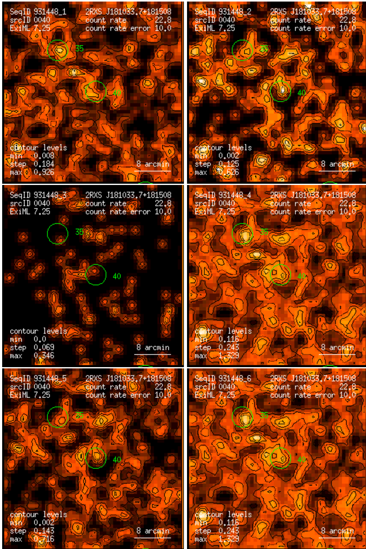
Figure 40: RASS 931448: detection 0040: band rate images, Gaussian filter: (1) PSPC channels 11 – 41, (2) 52 – 90, (3) 91 – 201, (4) 11 – 235, (5) 52 – 201, (6) 11 – 201. Broad band rates in counts/ks. Band rate contour levels in counts/ks/arcmin 2 .
