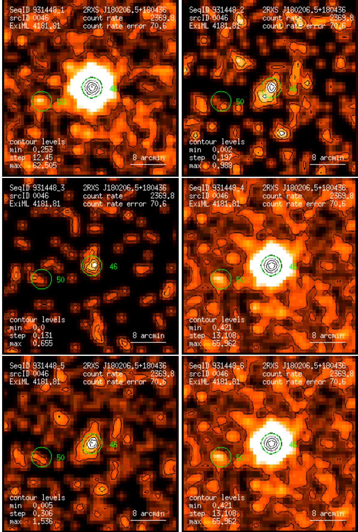
Figure 46: RASS 931448: detection 0046: band rate images, Gaussian filter: (1) PSPC channels 11 – 41, (2) 52 – 90, (3) 91 – 201, (4) 11 – 235, (5) 52 – 201, (6) 11 – 201. Broad band rates in counts/ks. Band rate contour levels in counts/ks/arcmin 2 .
