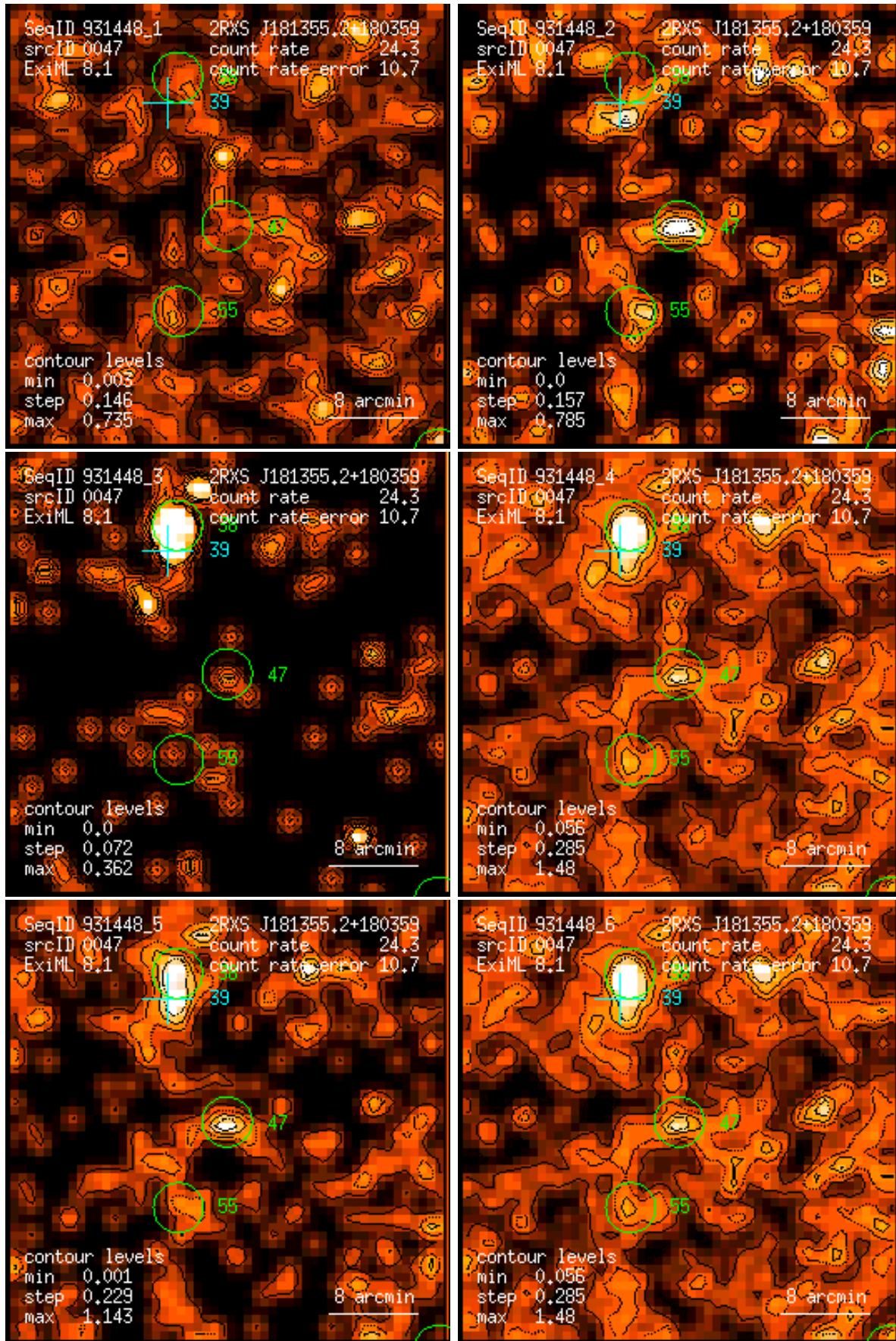
Figure 47: RASS 931448: detection 0047: band rate images, Gaussian filter: (1) PSPC channels 11 – 41, (2) 52 – 90, (3) 91 – 201, (4) 11 – 235, (5) 52 – 201, (6) 11 – 201. Broad band rates in counts/ks. Band rate contour levels in counts/ks/arcmin 2 .
