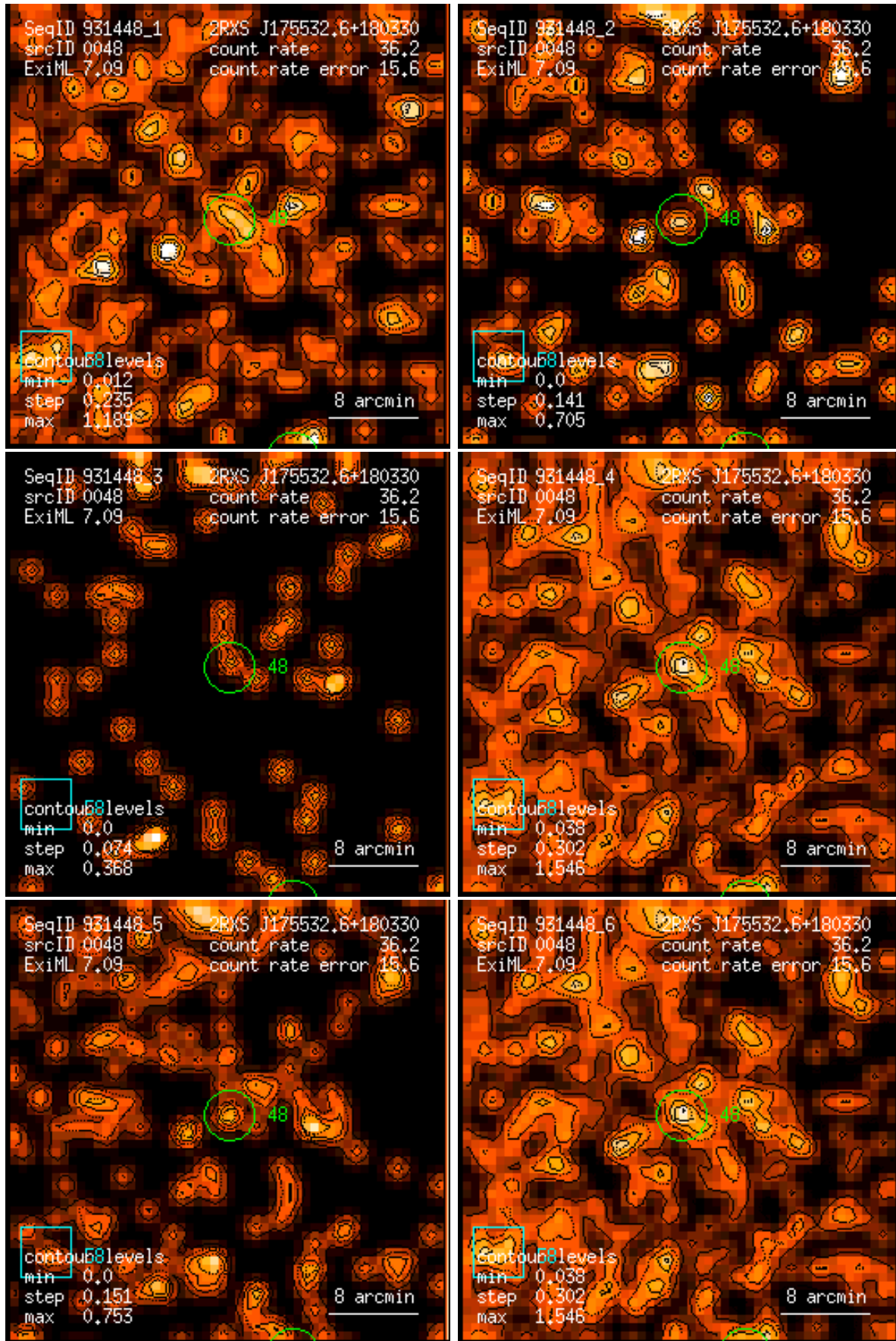
Figure 48: RASS 931448: detection 0048: band rate images, Gaussian filter: (1) PSPC channels 11 – 41, (2) 52 – 90, (3) 91 – 201, (4) 11 – 235, (5) 52 – 201, (6) 11 – 201. Broad band rates in counts/ks. Band rate contour levels in counts/ks/arcmin 2 .
