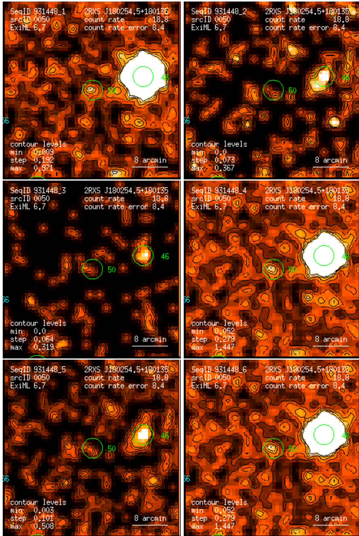
Figure 50: RASS 931448: detection 0050: band rate images, Gaussian filter: (1) PSPC channels 11 – 41, (2) 52 – 90, (3) 91 – 201, (4) 11 – 235, (5) 52 – 201, (6) 11 – 201. Broad band rates in counts/ks. Band rate contour levels in counts/ks/arcmin 2 .
