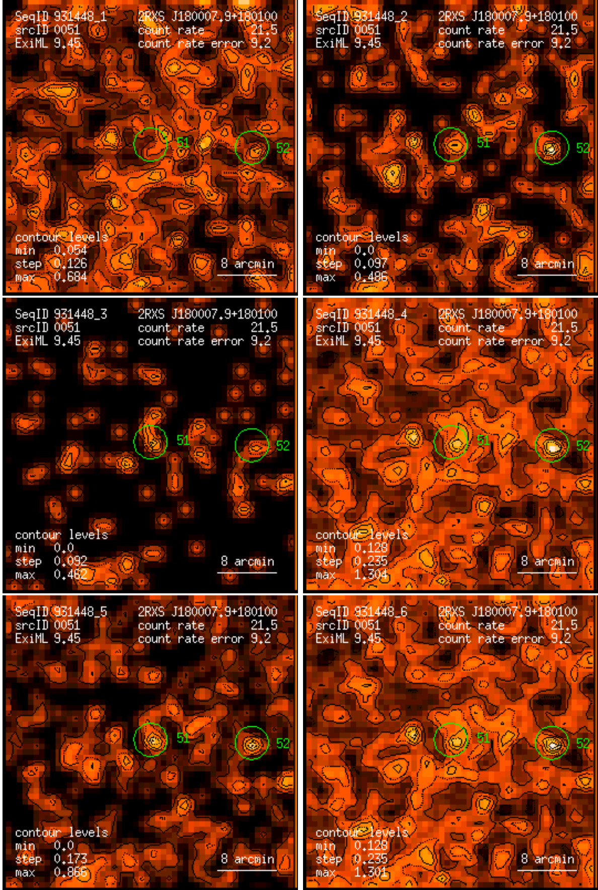
Figure 51: RASS 931448: detection 0051: band rate images, Gaussian filter: (1) PSPC channels 11 – 41, (2) 52 – 90, (3) 91 – 201, (4) 11 – 235, (5) 52 – 201, (6) 11 – 201. Broad band rates in counts/ks. Band rate contour levels in counts/ks/arcmin 2 .
