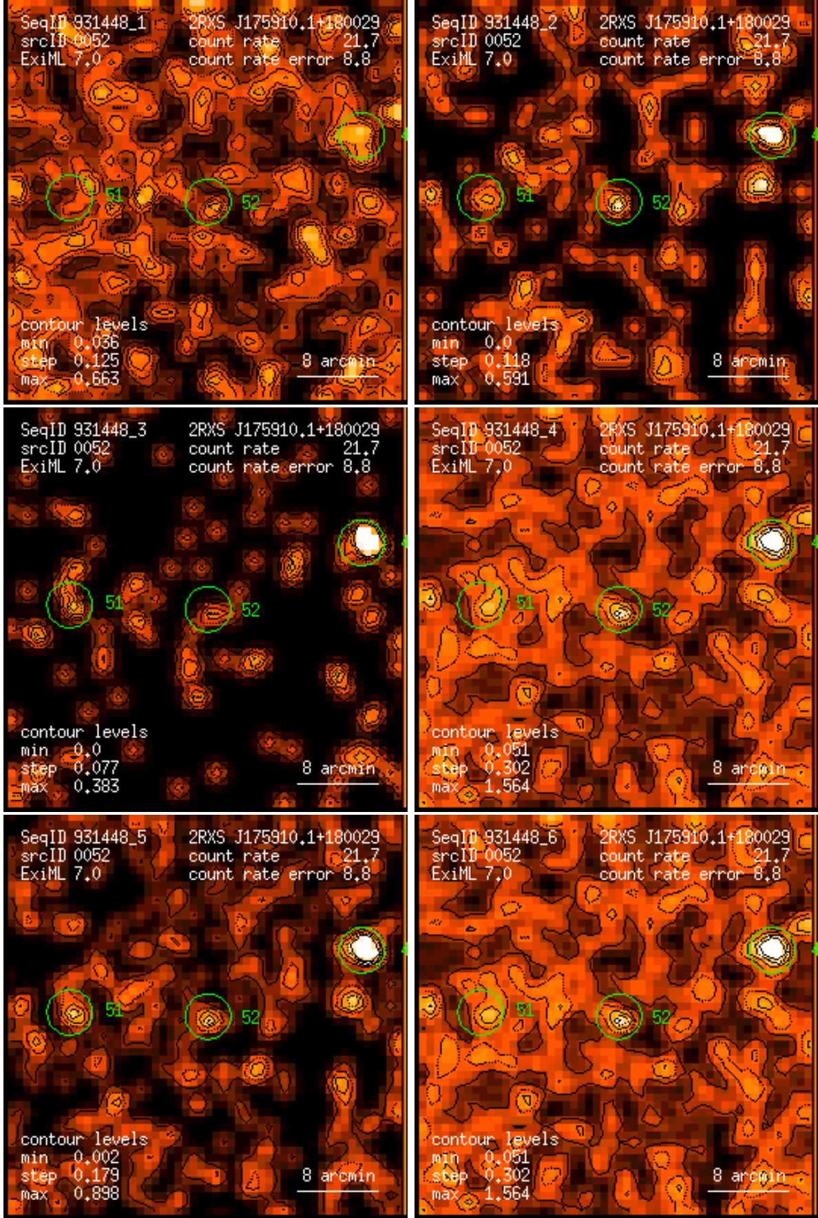
Figure 52: RASS 931448: detection 0052: band rate images, Gaussian filter: (1) PSPC channels 11 – 41, (2) 52 – 90, (3) 91 – 201, (4) 11 – 235, (5) 52 – 201, (6) 11 – 201. Broad band rates in counts/ks. Band rate contour levels in counts/ks/arcmin 2 .
