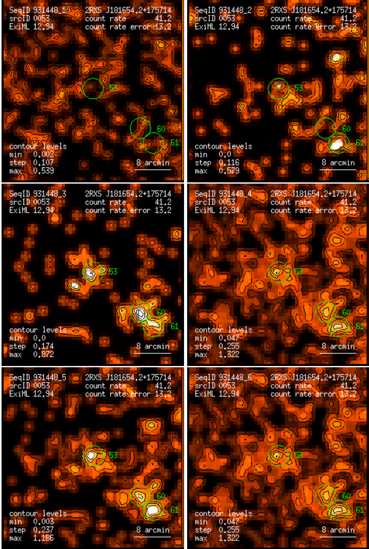
Figure 53: RASS 931448: detection 0053: band rate images, Gaussian filter: (1) PSPC channels 11 – 41, (2) 52 – 90, (3) 91 – 201, (4) 11 – 235, (5) 52 – 201, (6) 11 – 201. Broad band rates in counts/ks. Band rate contour levels in counts/ks/arcmin 2 .
