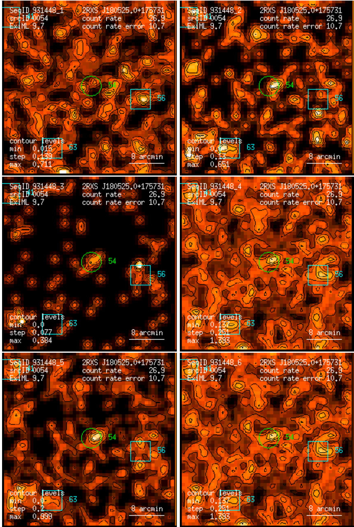
Figure 54: RASS 931448: detection 0054: band rate images, Gaussian filter: (1) PSPC channels 11 – 41, (2) 52 – 90, (3) 91 – 201, (4) 11 – 235, (5) 52 – 201, (6) 11 – 201. Broad band rates in counts/ks. Band rate contour levels in counts/ks/arcmin 2 .
