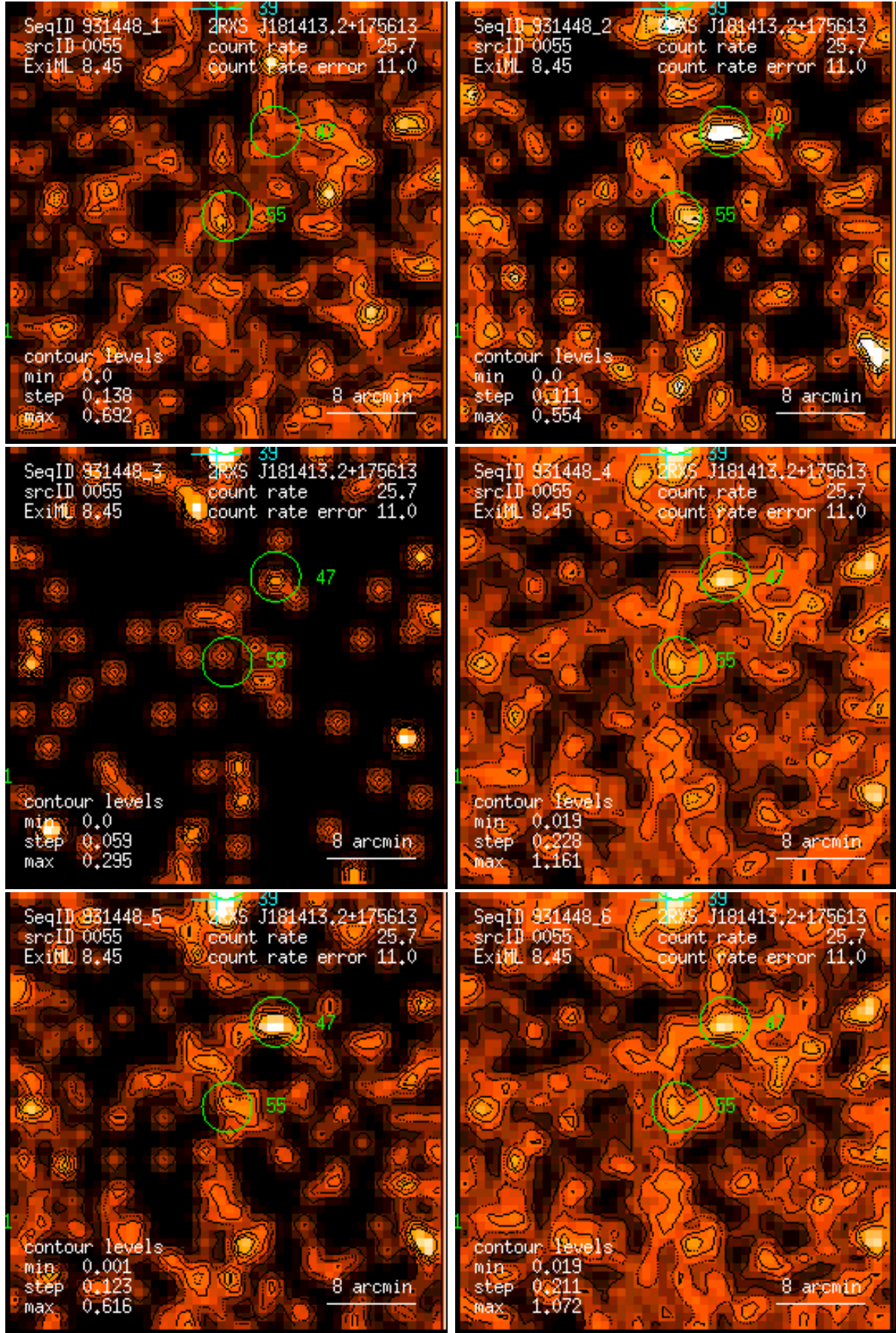
Figure 55: RASS 931448: detection 0055: band rate images, Gaussian filter: (1) PSPC channels 11 – 41, (2) 52 – 90, (3) 91 – 201, (4) 11 – 235, (5) 52 – 201, (6) 11 – 201. Broad band rates in counts/ks. Band rate contour levels in counts/ks/arcmin 2 .
