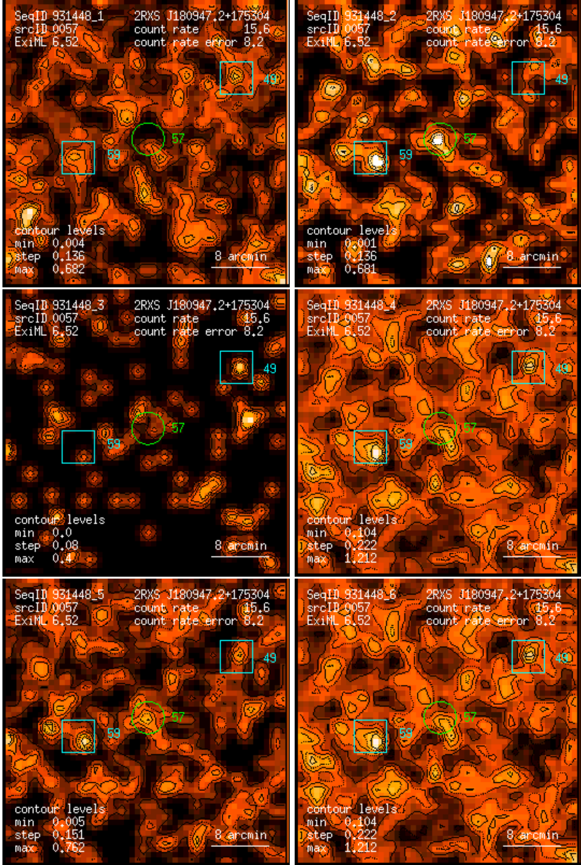
Figure 57: RASS 931448: detection 0057: band rate images, Gaussian filter: (1) PSPC channels 11 – 41, (2) 52 – 90, (3) 91 – 201, (4) 11 – 235, (5) 52 – 201, (6) 11 – 201. Broad band rates in counts/ks. Band rate contour levels in counts/ks/arcmin 2 .
