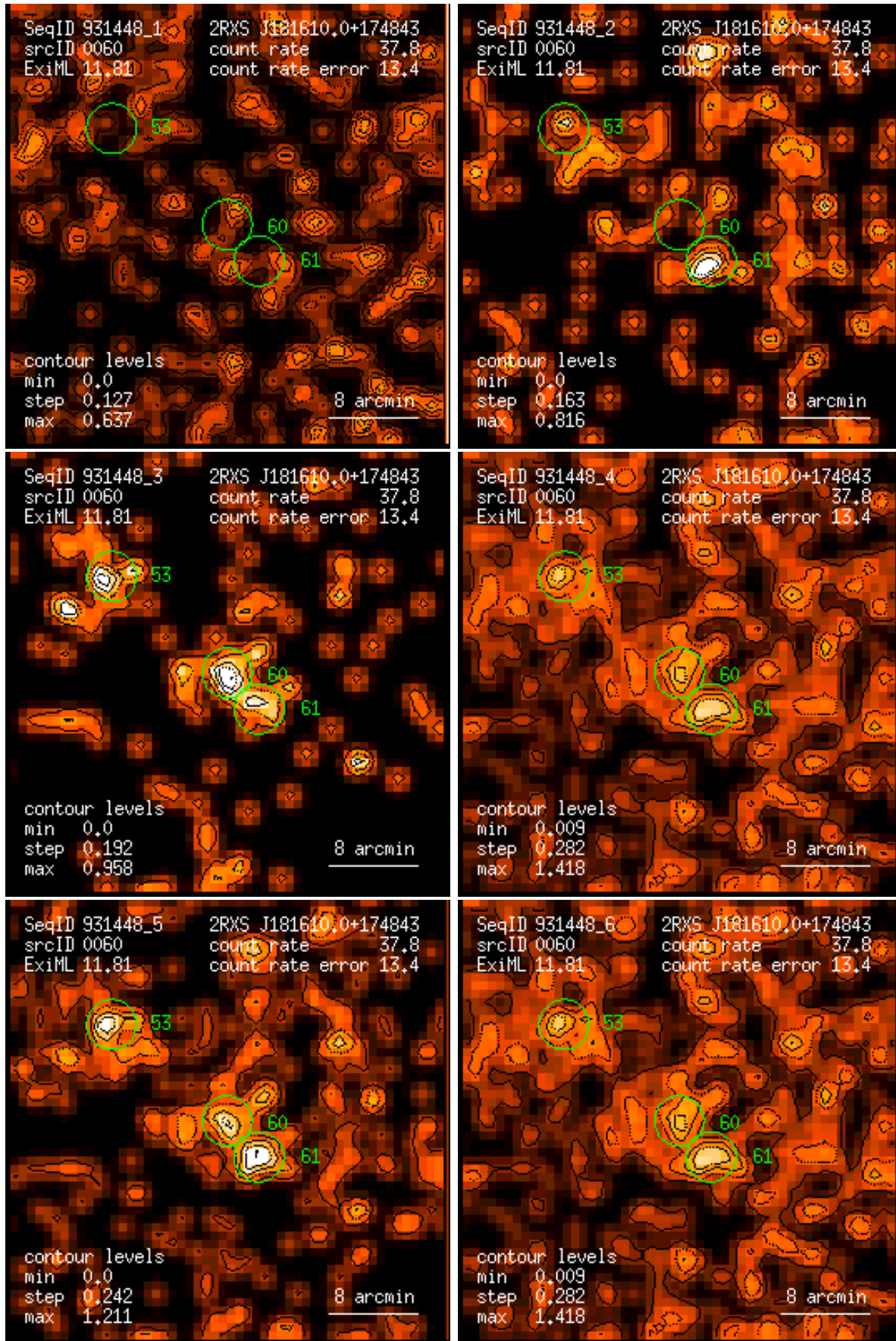
Figure 60: RASS 931448: detection 0060: band rate images, Gaussian filter: (1) PSPC channels 11 – 41, (2) 52 – 90, (3) 91 – 201, (4) 11 – 235, (5) 52 – 201, (6) 11 – 201. Broad band rates in counts/ks. Band rate contour levels in counts/ks/arcmin 2 .
