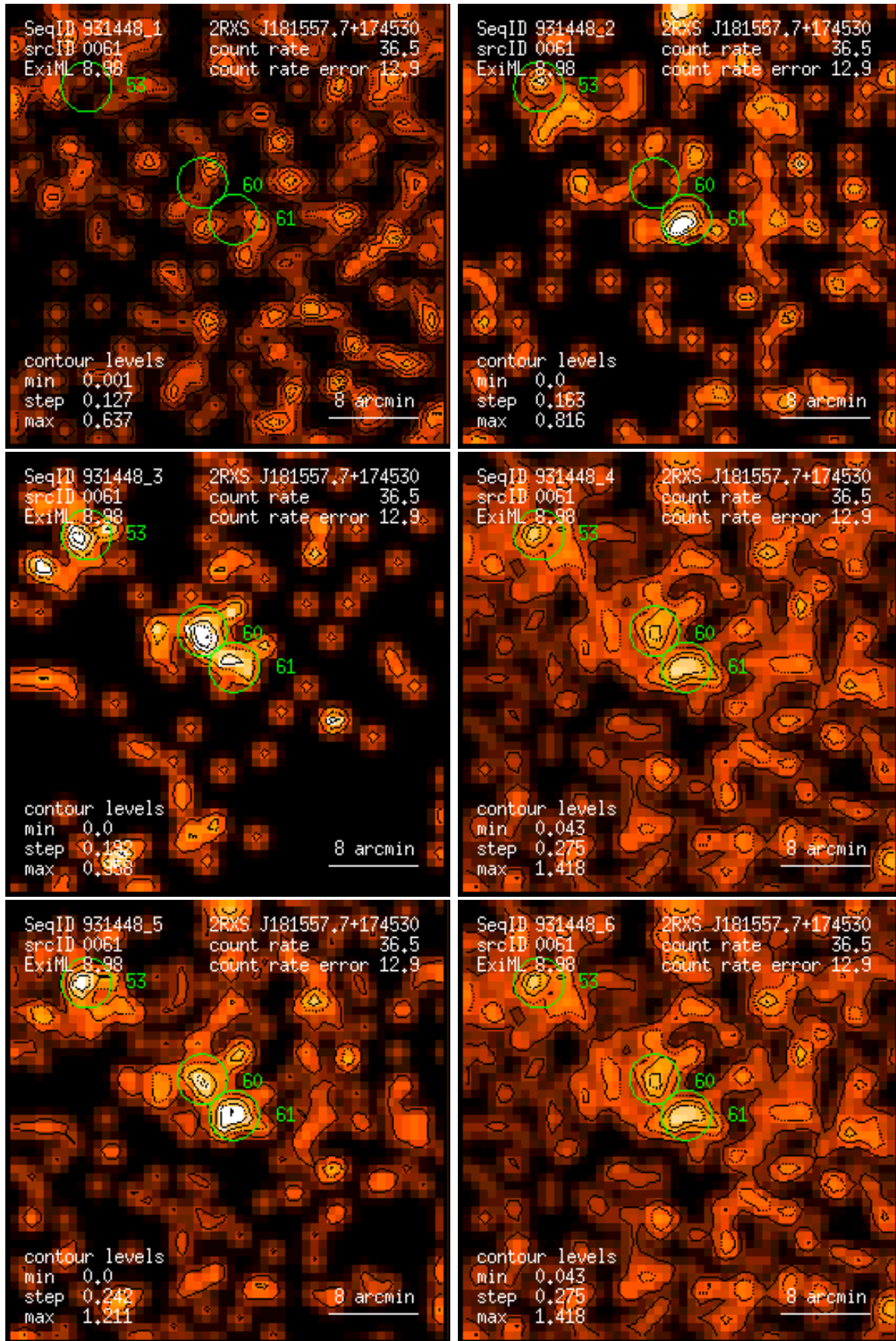
Figure 61: RASS 931448: detection 0061: band rate images, Gaussian filter: (1) PSPC channels 11 – 41, (2) 52 – 90, (3) 91 – 201, (4) 11 – 235, (5) 52 – 201, (6) 11 – 201. Broad band rates in counts/ks. Band rate contour levels in counts/ks/arcmin 2 .
