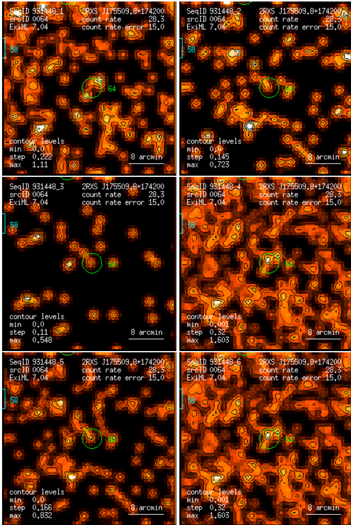
Figure 64: RASS 931448: detection 0064: band rate images, Gaussian filter: (1) PSPC channels 11 – 41, (2) 52 – 90, (3) 91 – 201, (4) 11 – 235, (5) 52 – 201, (6) 11 – 201. Broad band rates in counts/ks. Band rate contour levels in counts/ks/arcmin 2 .
