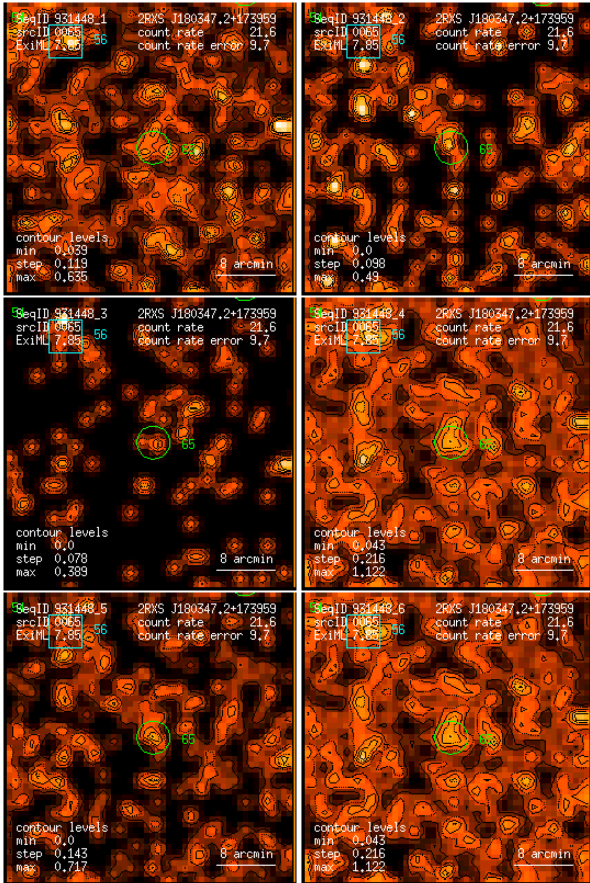
Figure 65: RASS 931448: detection 0065: band rate images, Gaussian filter: (1) PSPC channels 11 – 41, (2) 52 – 90, (3) 91 – 201, (4) 11 – 235, (5) 52 – 201, (6) 11 – 201. Broad band rates in counts/ks. Band rate contour levels in counts/ks/arcmin 2 .
