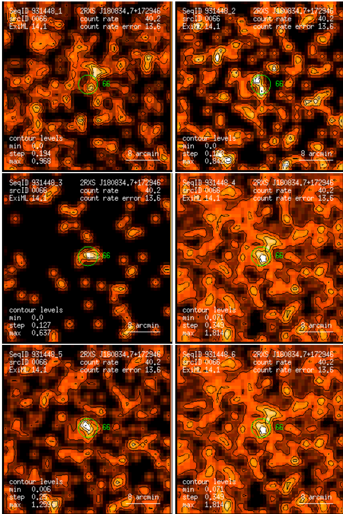
Figure 66: RASS 931448: detection 0066: band rate images, Gaussian filter: (1) PSPC channels 11 – 41, (2) 52 – 90, (3) 91 – 201, (4) 11 – 235, (5) 52 – 201, (6) 11 – 201. Broad band rates in counts/ks. Band rate contour levels in counts/ks/arcmin 2 .
