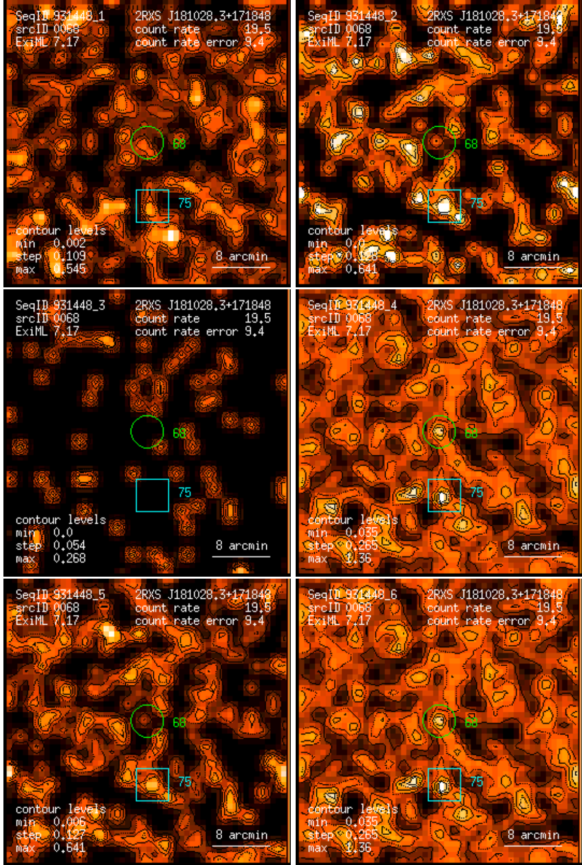
Figure 68: RASS 931448: detection 0068: band rate images, Gaussian filter: (1) PSPC channels 11 – 41, (2) 52 – 90, (3) 91 – 201, (4) 11 – 235, (5) 52 – 201, (6) 11 – 201. Broad band rates in counts/ks. Band rate contour levels in counts/ks/arcmin 2 .
