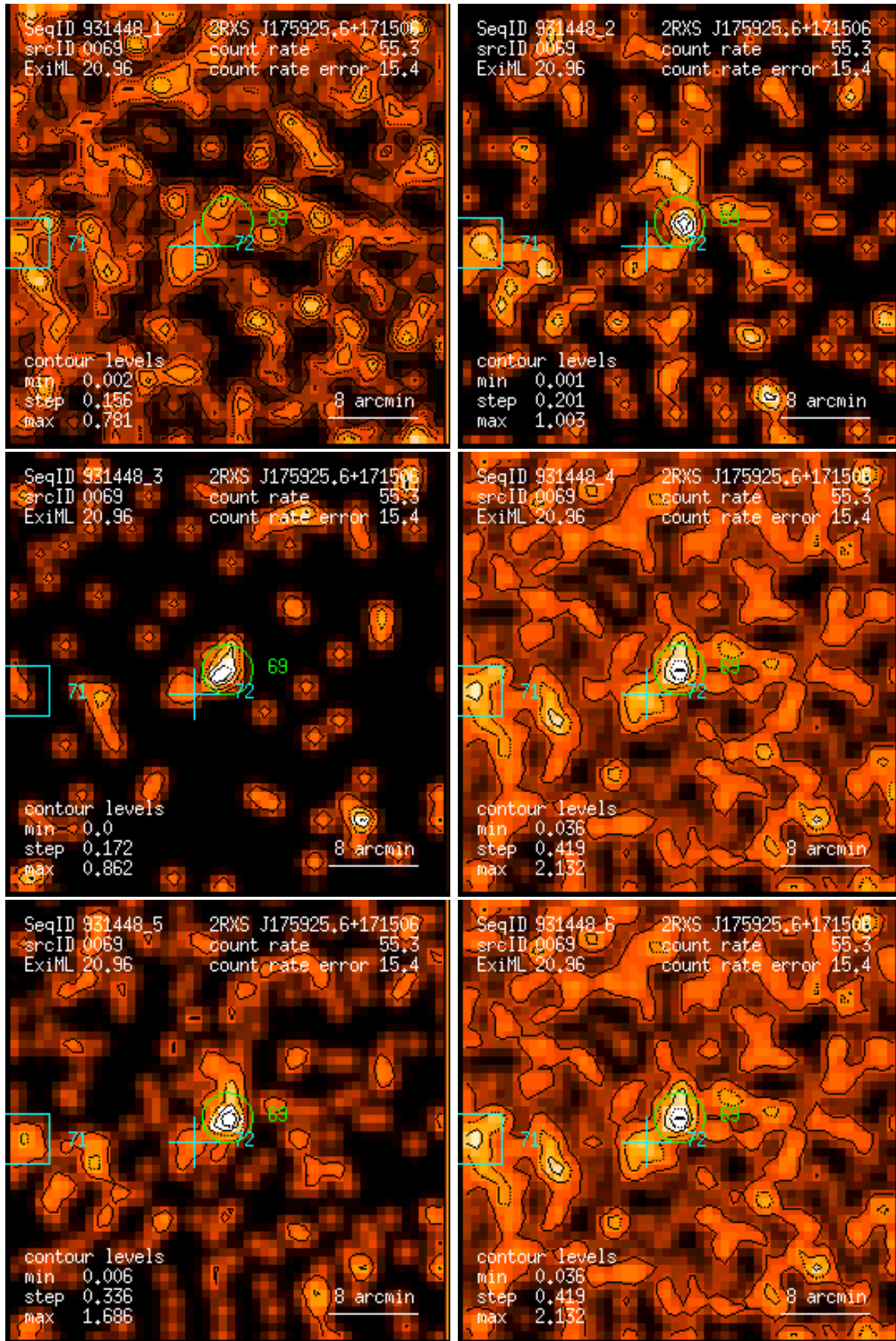
Figure 69: RASS 931448: detection 0069: band rate images, Gaussian filter: (1) PSPC channels 11 – 41, (2) 52 – 90, (3) 91 – 201, (4) 11 – 235, (5) 52 – 201, (6) 11 – 201. Broad band rates in counts/ks. Band rate contour levels in counts/ks/arcmin 2 .
