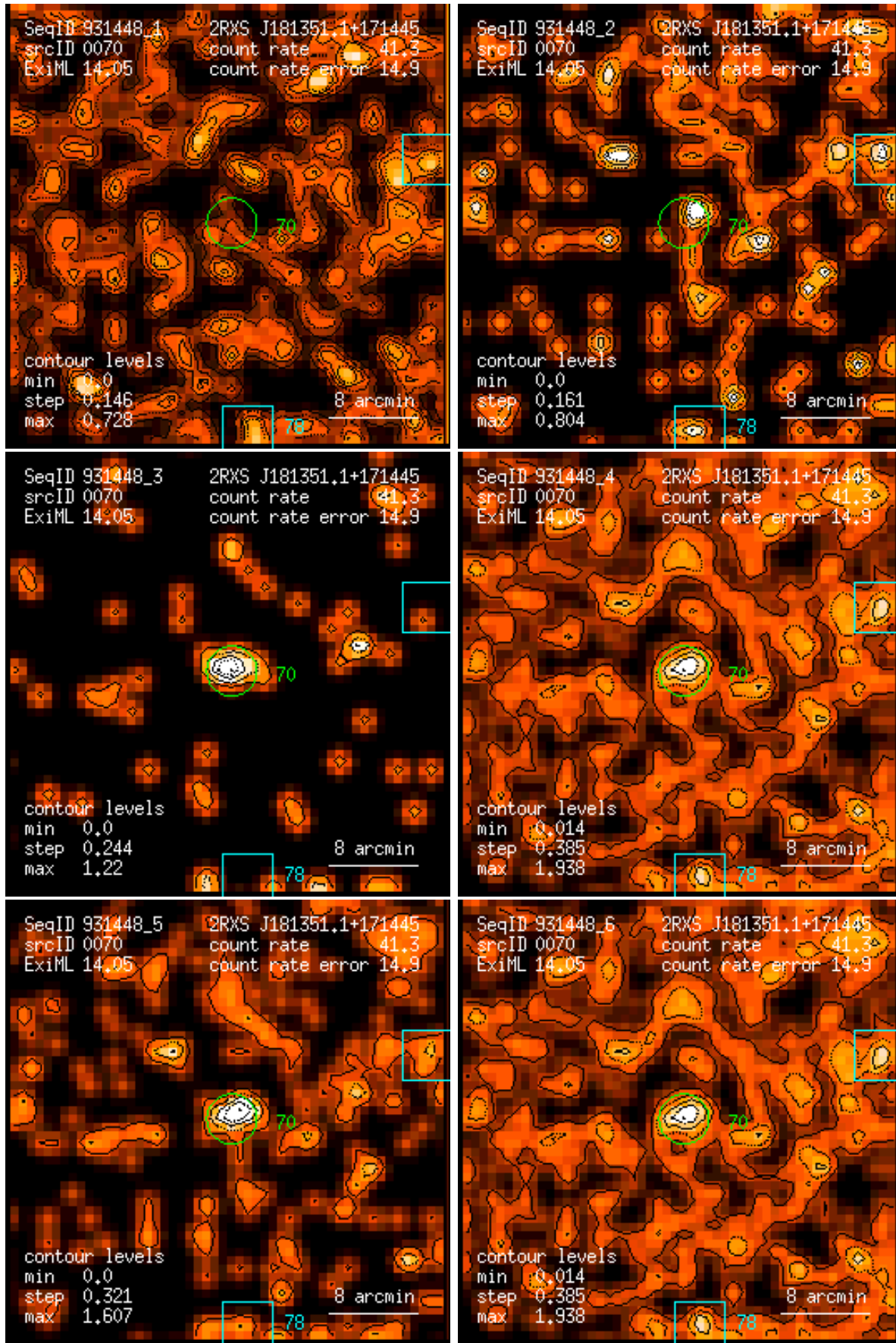
Figure 70: RASS 931448: detection 0070: band rate images, Gaussian filter: (1) PSPC channels 11 – 41, (2) 52 – 90, (3) 91 – 201, (4) 11 – 235, (5) 52 – 201, (6) 11 – 201. Broad band rates in counts/ks. Band rate contour levels in counts/ks/arcmin 2 .
