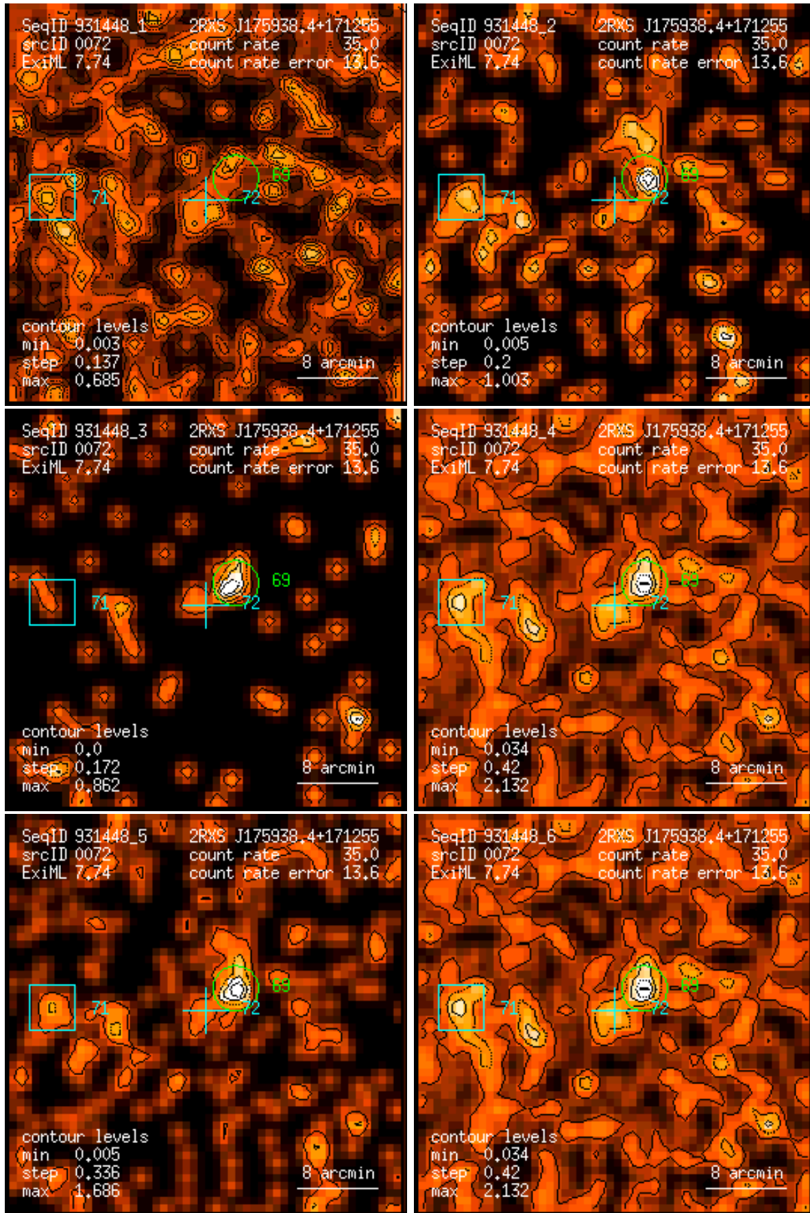
Figure 72: RASS 931448: detection 0072: band rate images, Gaussian filter: (1) PSPC channels 11 – 41, (2) 52 – 90, (3) 91 – 201, (4) 11 – 235, (5) 52 – 201, (6) 11 – 201. Broad band rates in counts/ks. Band rate contour levels in counts/ks/arcmin 2 .
