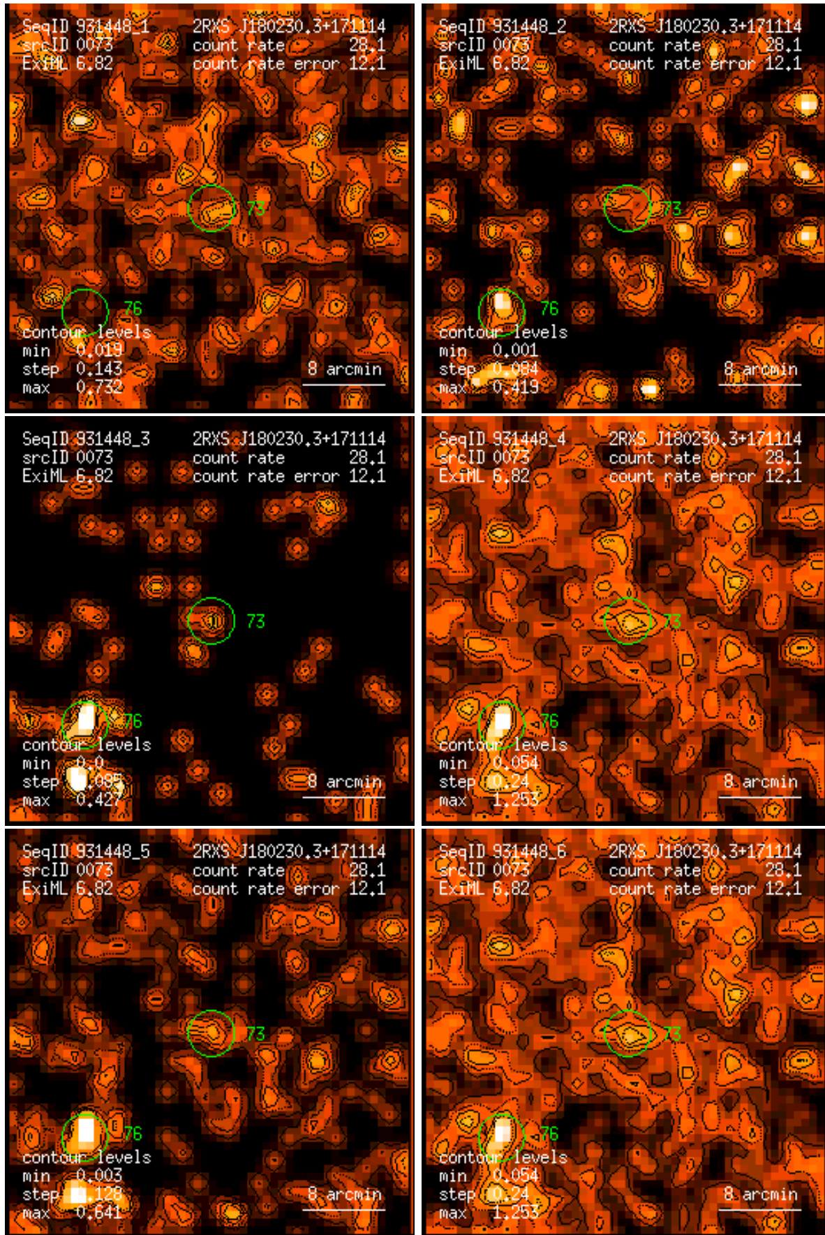
Figure 73: RASS 931448: detection 0073: band rate images, Gaussian filter: (1) PSPC channels 11 – 41, (2) 52 – 90, (3) 91 – 201, (4) 11 – 235, (5) 52 – 201, (6) 11 – 201. Broad band rates in counts/ks. Band rate contour levels in counts/ks/arcmin 2 .
