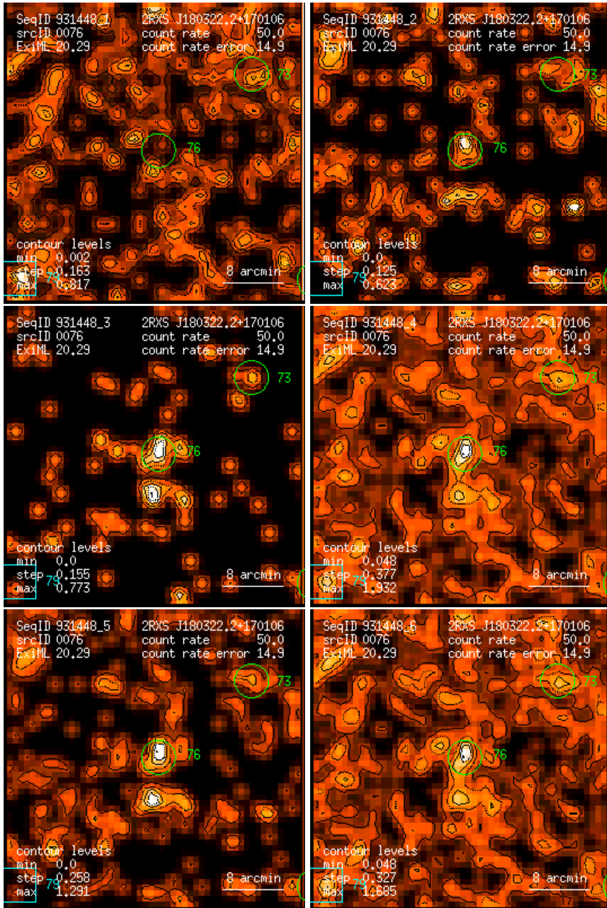
Figure 76: RASS 931448: detection 0076: band rate images, Gaussian filter: (1) PSPC channels 11 – 41, (2) 52 – 90, (3) 91 – 201, (4) 11 – 235, (5) 52 – 201, (6) 11 – 201. Broad band rates in counts/ks. Band rate contour levels in counts/ks/arcmin 2 .
