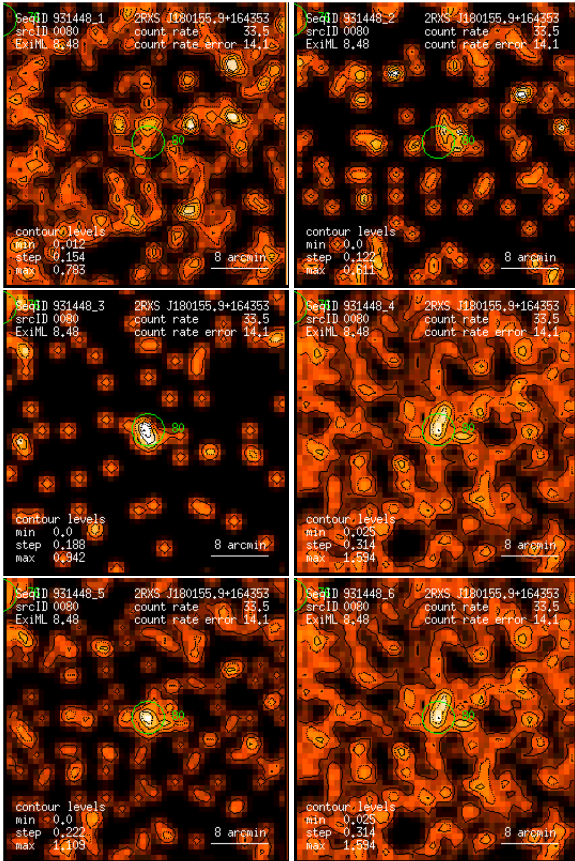
Figure 80: RASS 931448: detection 0080: band rate images, Gaussian filter: (1) PSPC channels 11 – 41, (2) 52 – 90, (3) 91 – 201, (4) 11 – 235, (5) 52 – 201, (6) 11 – 201. Broad band rates in counts/ks. Band rate contour levels in counts/ks/arcmin 2 .
