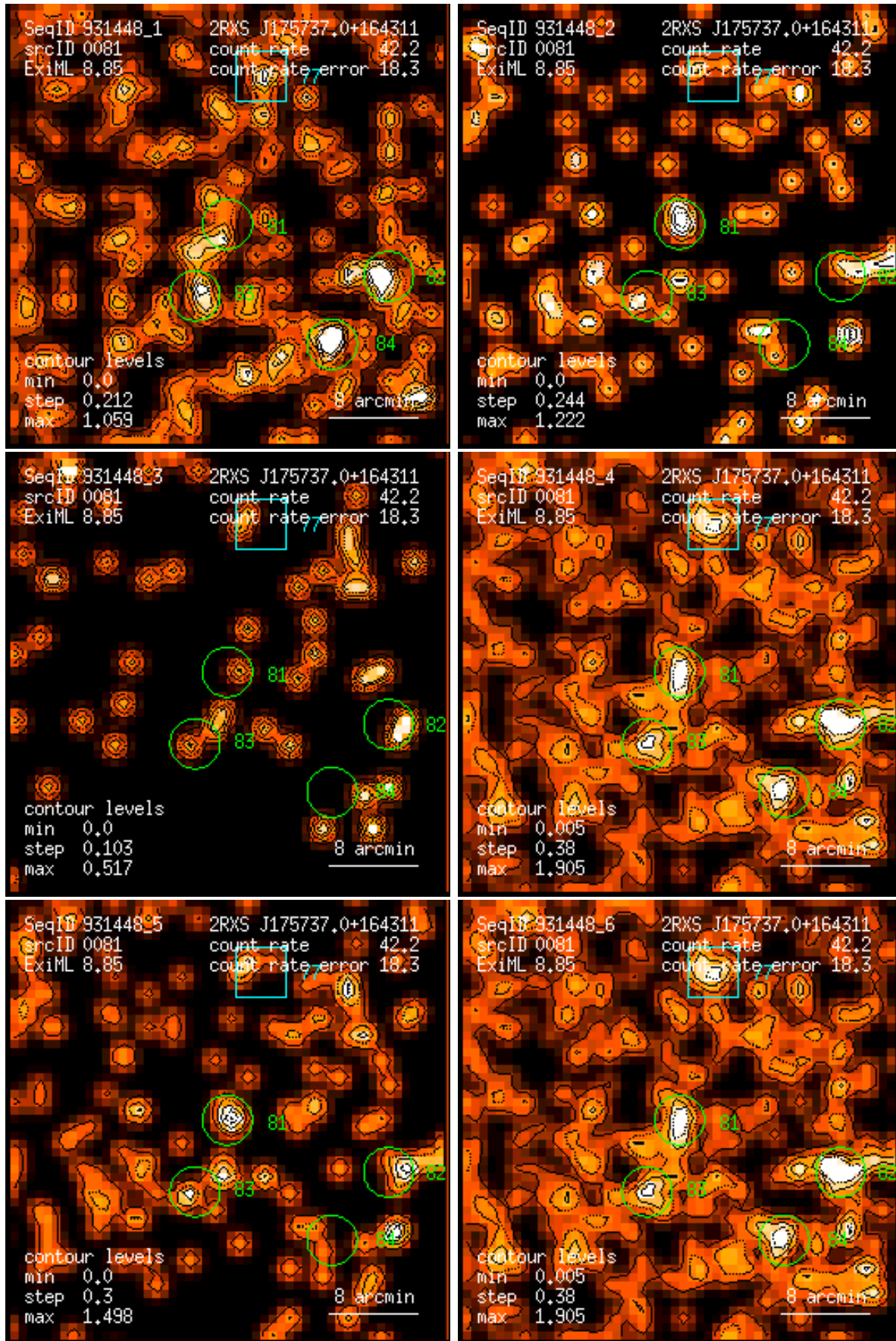
Figure 81: RASS 931448: detection 0081: band rate images, Gaussian filter: (1) PSPC channels 11 – 41, (2) 52 – 90, (3) 91 – 201, (4) 11 – 235, (5) 52 – 201, (6) 11 – 201. Broad band rates in counts/ks. Band rate contour levels in counts/ks/arcmin 2 .
