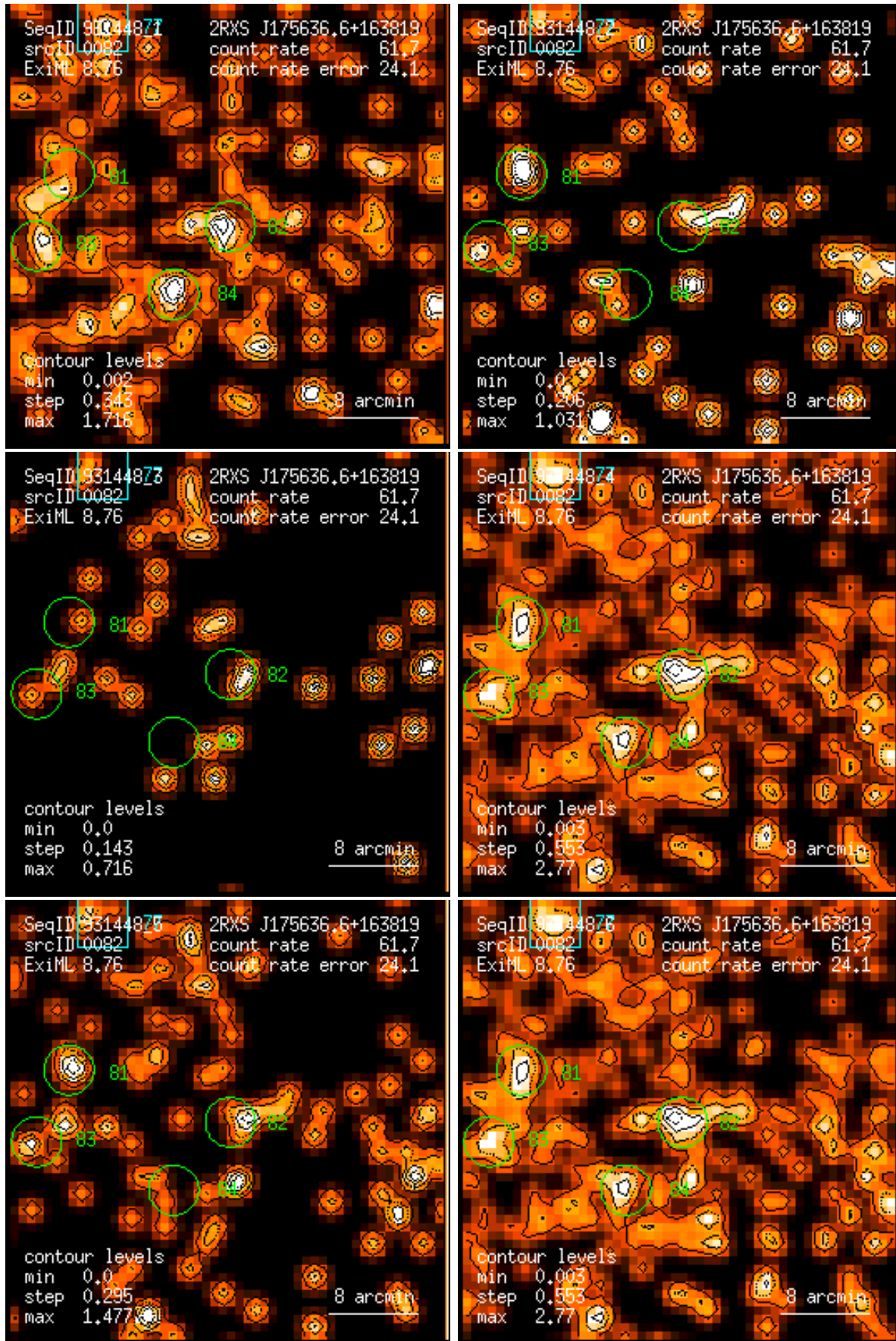
Figure 82: RASS 931448: detection 0082: band rate images, Gaussian filter: (1) PSPC channels 11 – 41, (2) 52 – 90, (3) 91 – 201, (4) 11 – 235, (5) 52 – 201, (6) 11 – 201. Broad band rates in counts/ks. Band rate contour levels in counts/ks/arcmin 2 .
